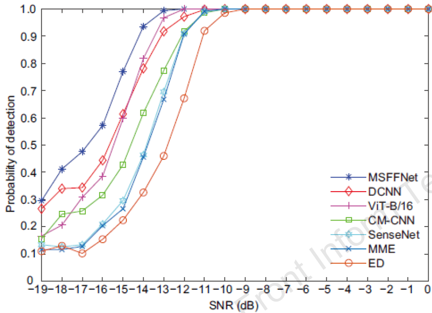
Fig. 7 P_d -SNR curves of the MSFFNet and six comparison methods
