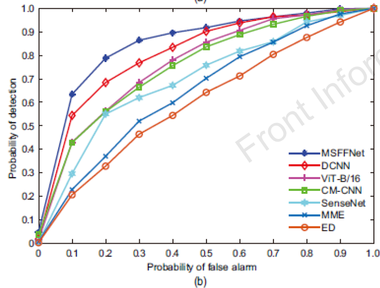
Fig. 12 Detection performance of spectrum sensing methods under colored noise: (a) P_d -SNR curves; (b) ROC curves
