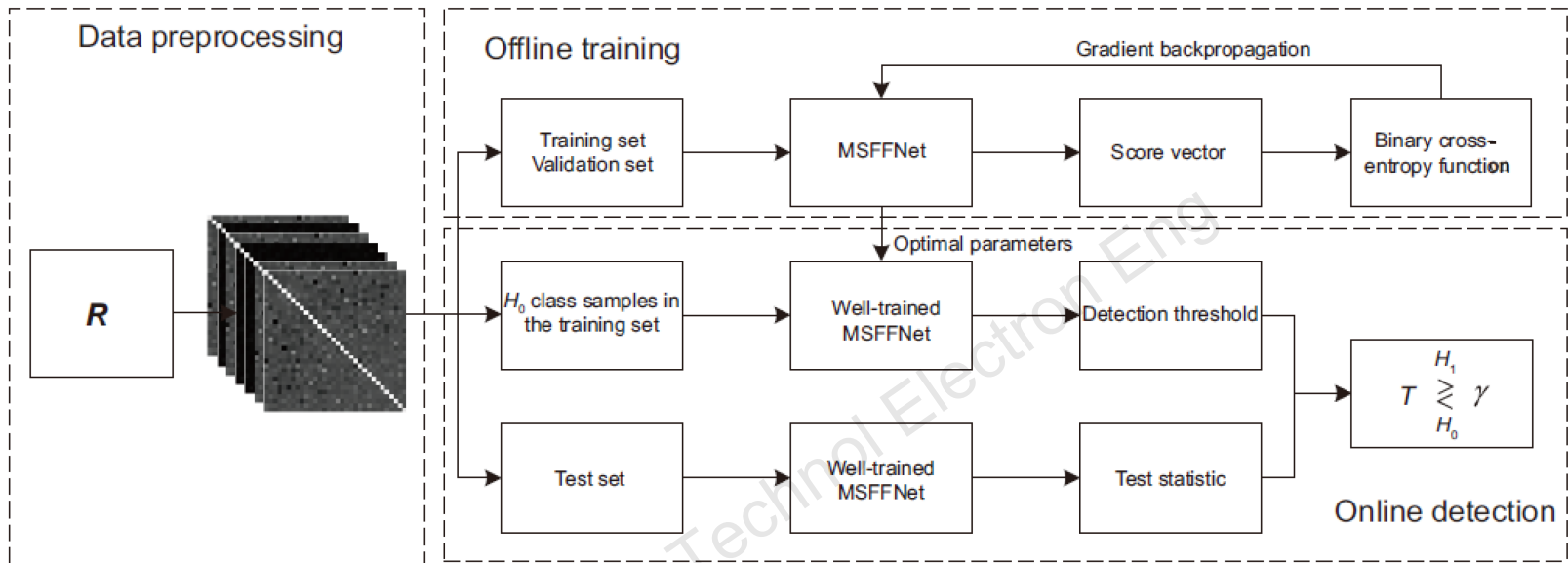
Fig. 1 Spectrum sensing system based on MSFFNet
