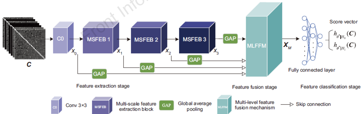
Fig. 3 MSFFNet model structure
