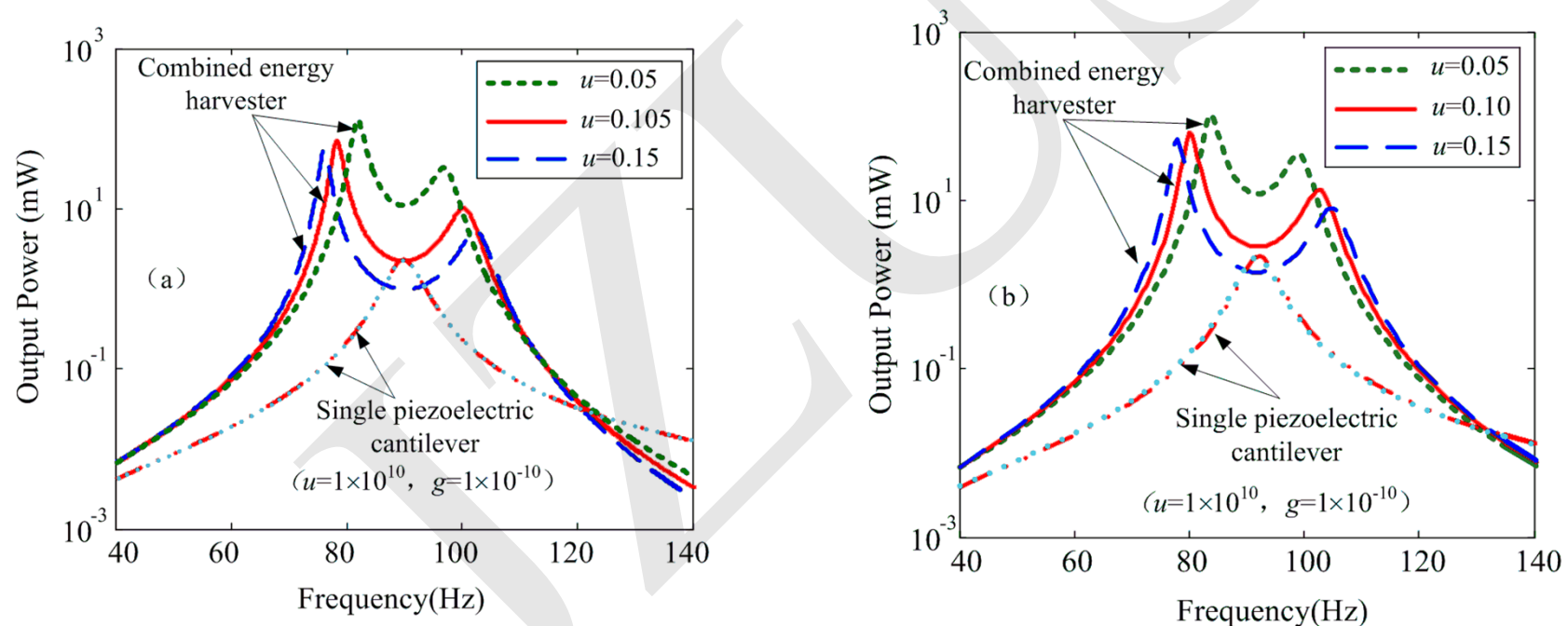
Fig. 3 Output power for single and combined energy harvester with different mass ratios u . (a) from numerical calculation; (b) from system-level FEA
