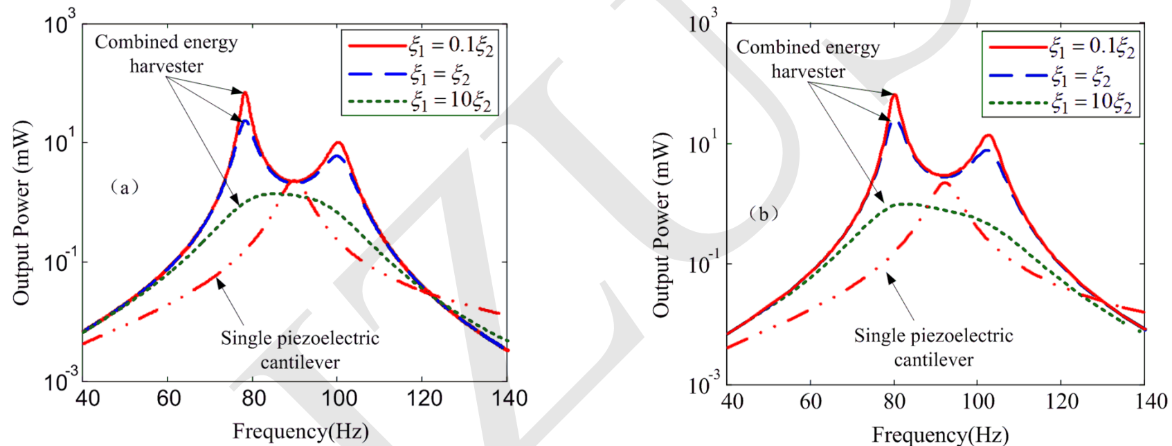
Fig. 4 Output power for single and combined energy harvester with different damping ratios. (a) from numerical calculation; (b) from system-level FEA
