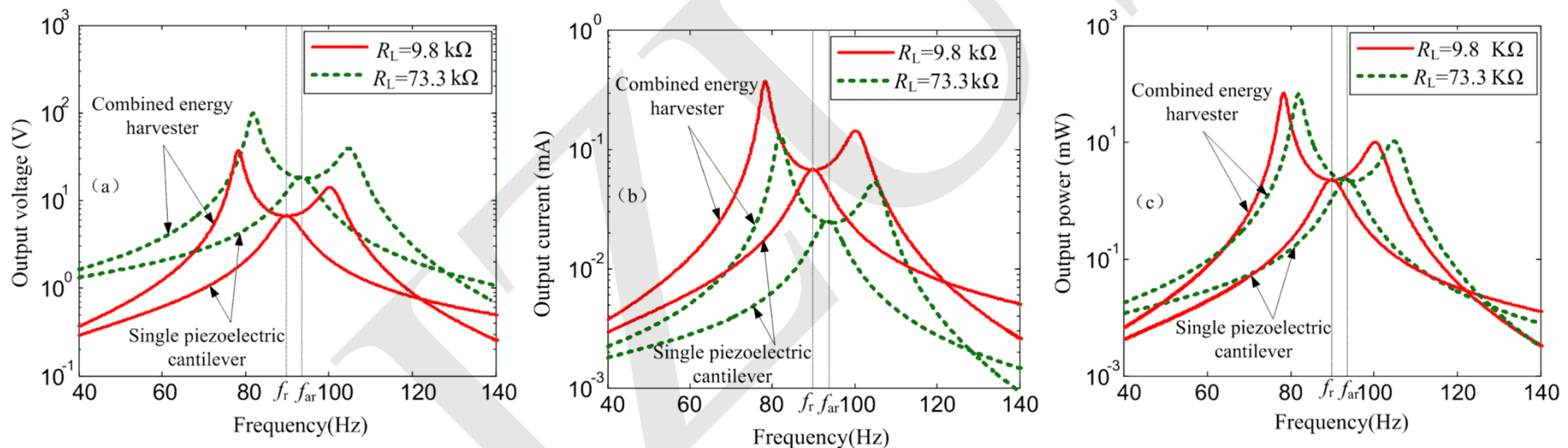
Fig. 5 Electrical outputs vs. vibration frequency for two different load resistances. (a) output voltage; (b) output current; (c) output power
