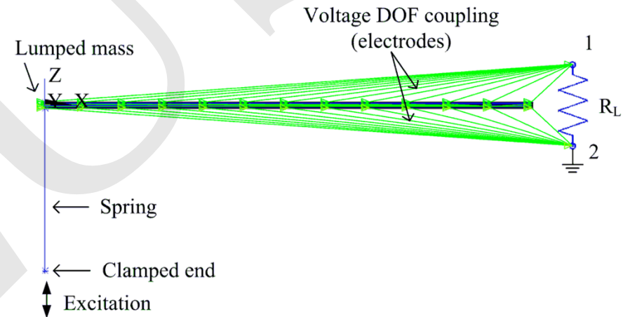
Fig. 2 Finite element model of the energy harvester combining a piezoelectric cantilever and an SDOF elastic system
