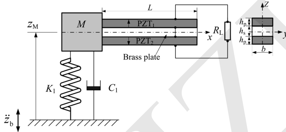
Fig. 1 Model of energy harvester combining a piezoelectric cantilever and an SDOF elastic system
