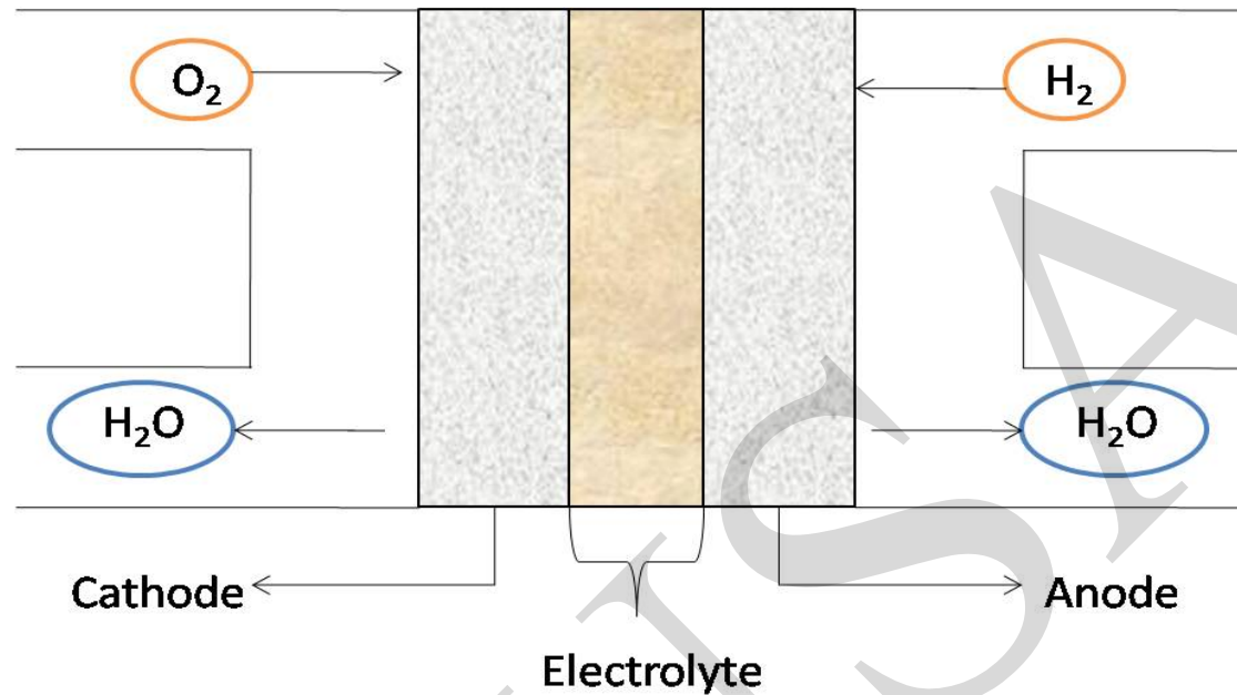
Fig. 1 Schematic of a solid oxide fuel cell
