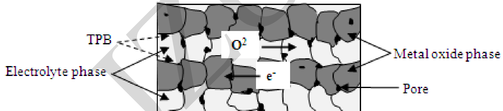
Fig. 2 Simplified schematic of the mechanism of electronic and ionic conductions in the composite cathode
