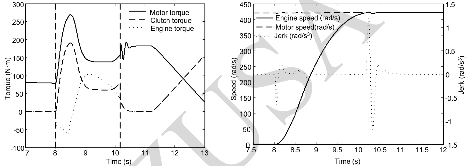
Fig. 3 Simulation results with system uncertainties and time delays using proposed engine side control and proposed motor side control
