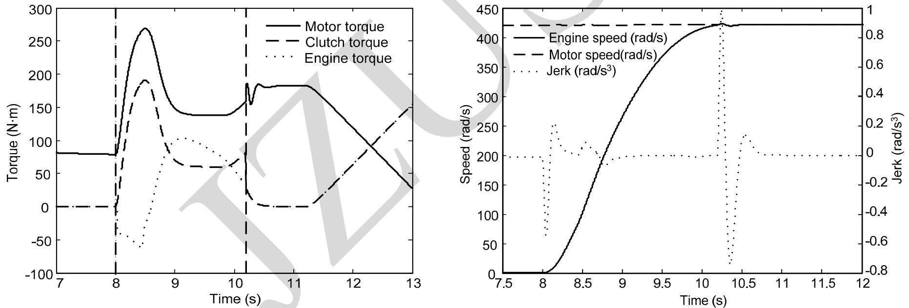
Fig. 2 Nominal simulation results with proposed engine side control and proposed motor side control
