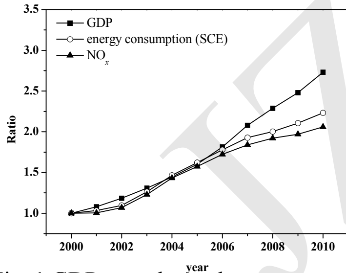
Fig. 1 GDP growth trends, energy consumption and \text{NO}_x emissions of China.
