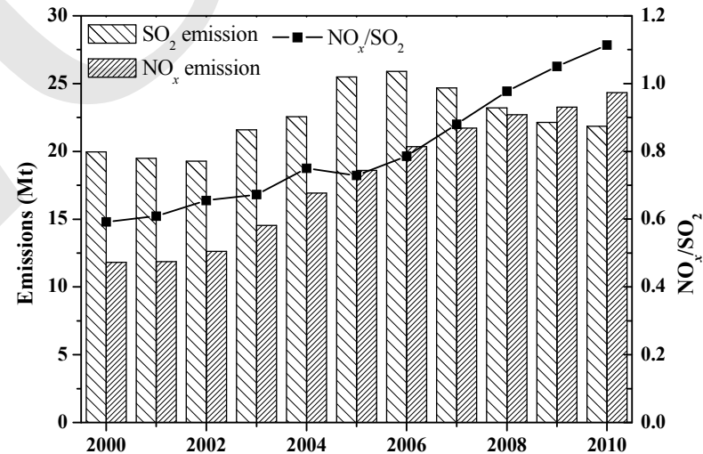
Fig. 2 Comparison of \text{SO}_2 and \text{NO}_x emissions in China.
