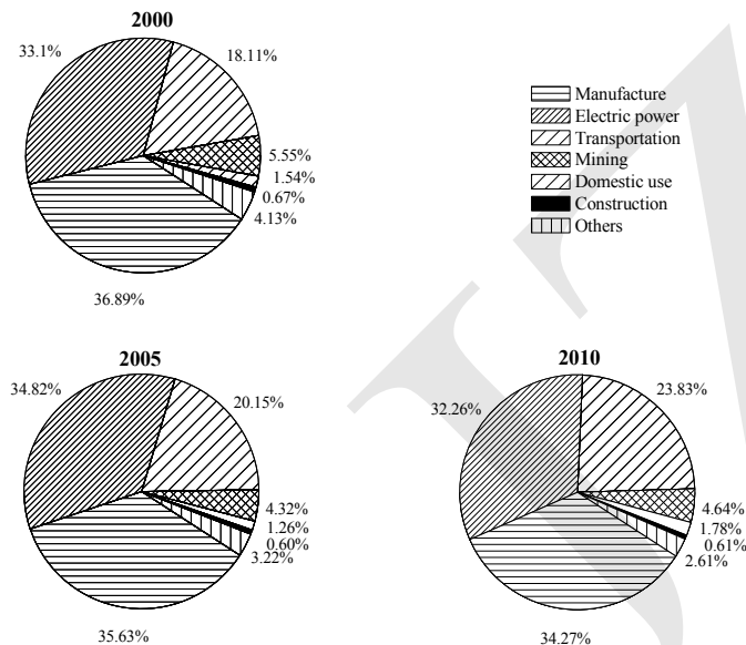
Fig. 4 Economic sector shares on \text{NO}_x emissions in 2000, 2005, and 2010
