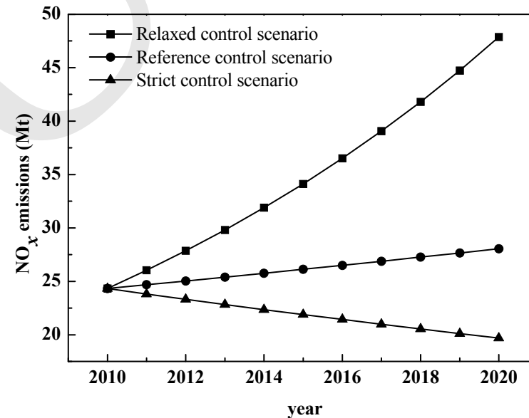
Fig 9. Prediction of \text{NO}_x Emissions in China over 2011-2020.
