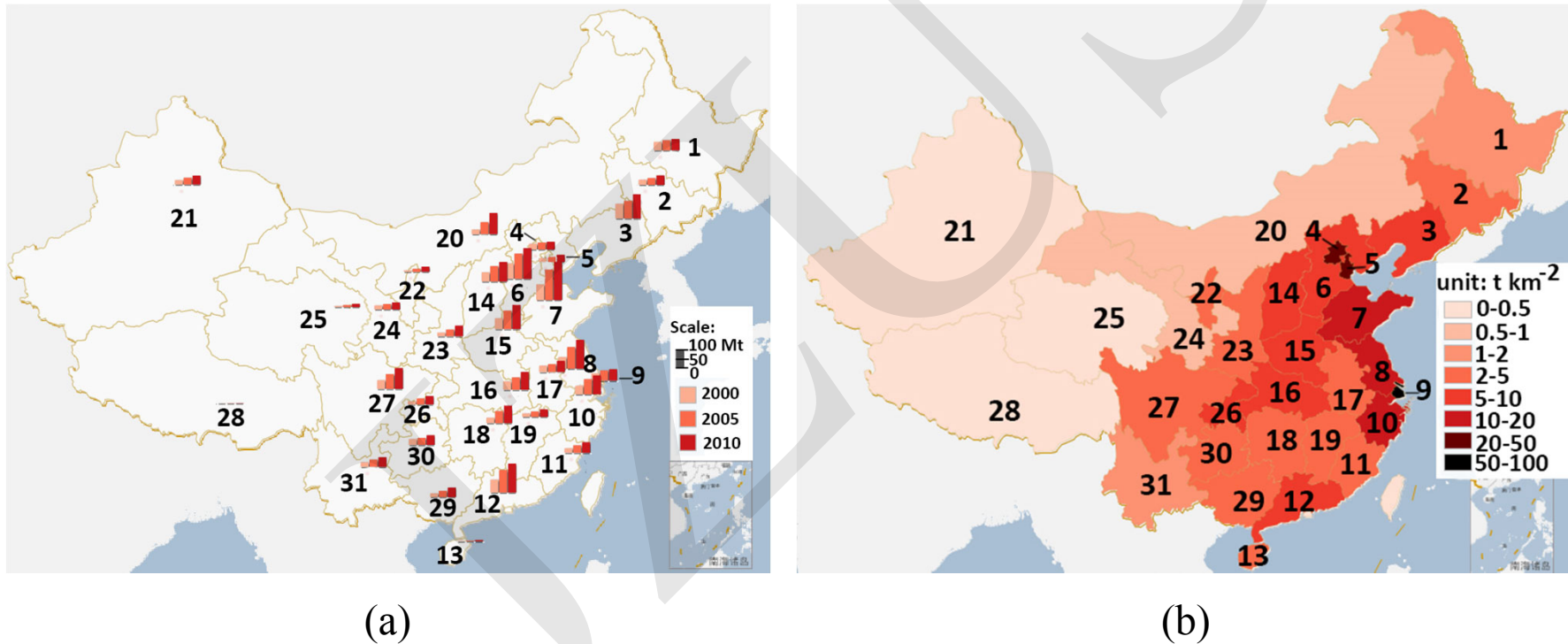
Fig. 3 NO x emission trends (a) and distributions (b) of different provinces in China
