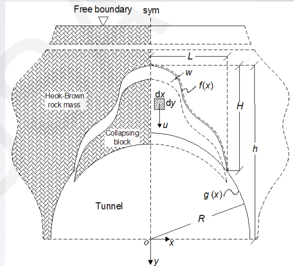
Fig. 1 Collapsing pattern of the deep tunnels
