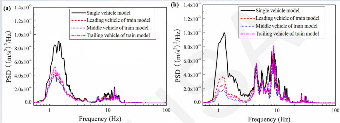
(a) Car body vertical acceleration PSD; (b) Car body lateral acceleration PSD
