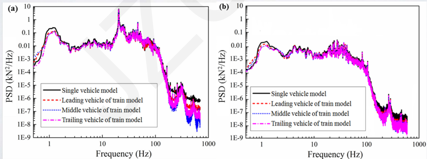
(a) Wheel/rail vertical force PSD; (b) Wheel/rail lateral force PSD
