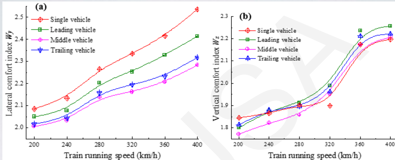
(a) Lateral Sperling comfort index; (b) Vertical Sperling comfort index
