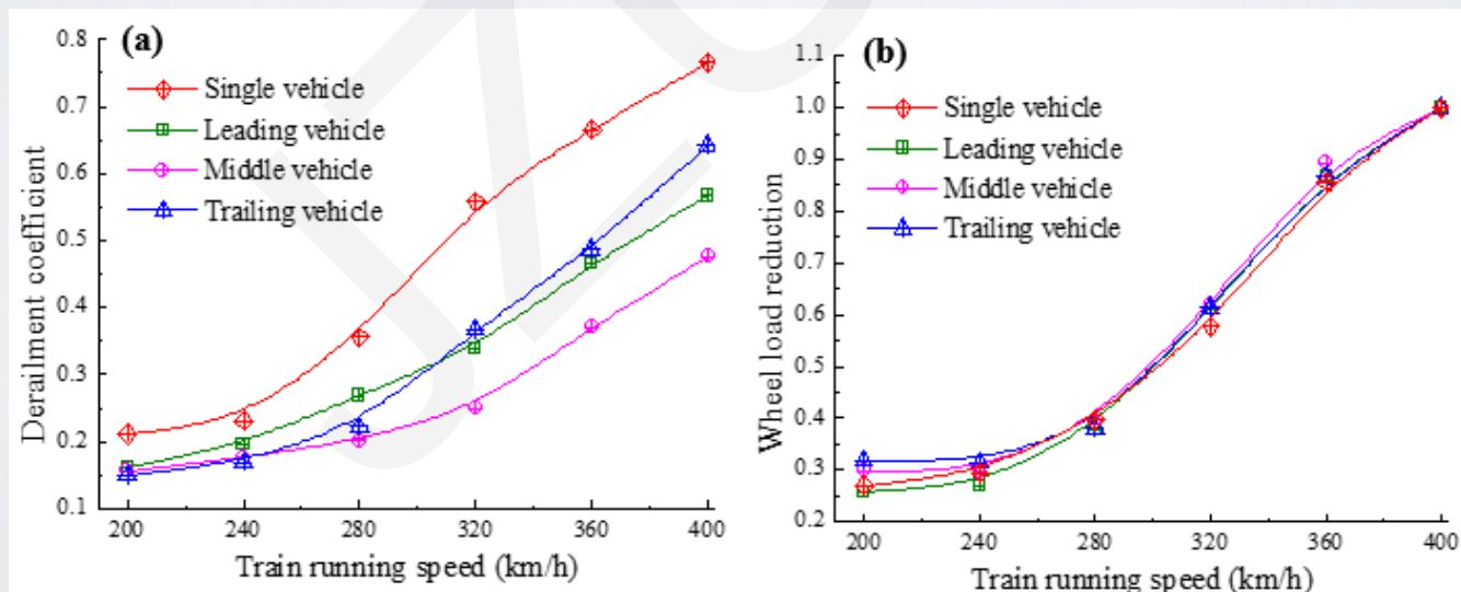
(a) Derailment coefficient; (b) Wheel load reduction
