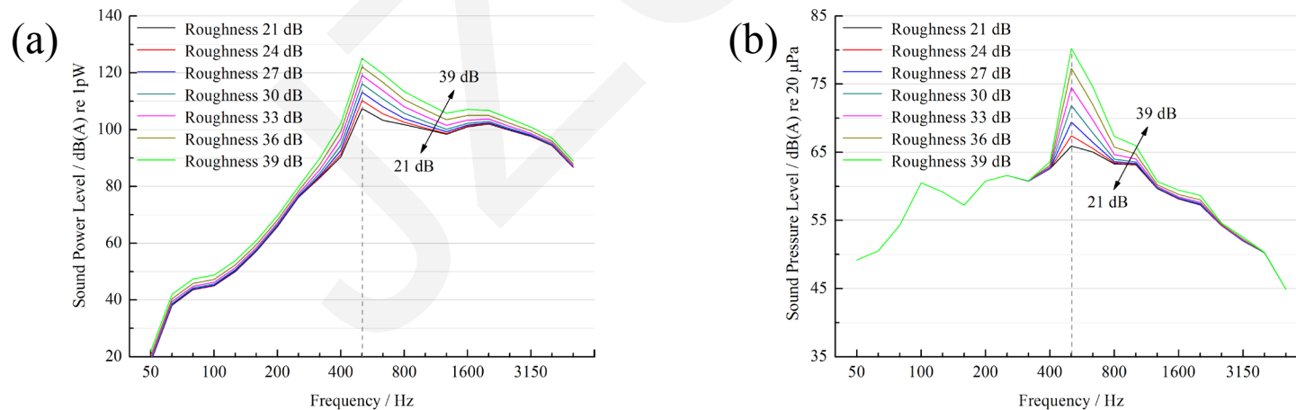
Fig. 15 Different roughness levels: (a) wheel/rail noise, (b) interior noise.
