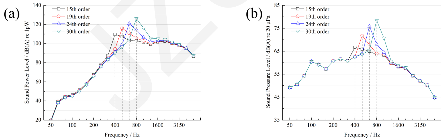
Fig. 13 Different polygon order: (a) wheel/rail noise, (b) interior noise.
