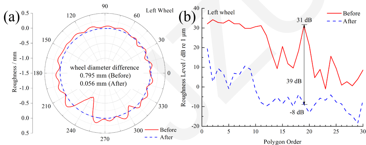
Fig. 3 (a) wheel roughness, (b) polygon order before and after the re-profiling
