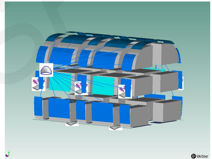
Fig. 9 The hybrid FE-SEA simulation model of coach end
