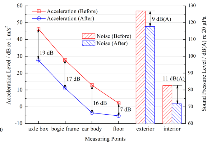
Fig. 4 Noise and vibration before and after the re-profiling
