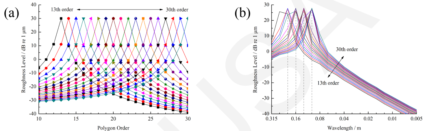
Fig. 12 Different polygon order: (a) polygon roughness levels characterized by order, (b) polygon roughness levels characterized with the wavelength
