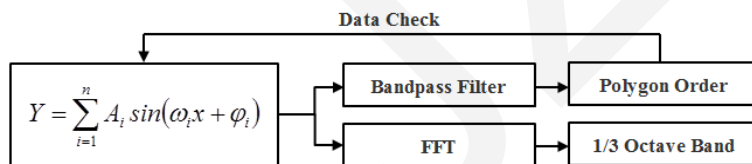
Fig. 11 The MATLAB code technique routine for creating wheel polygon data
