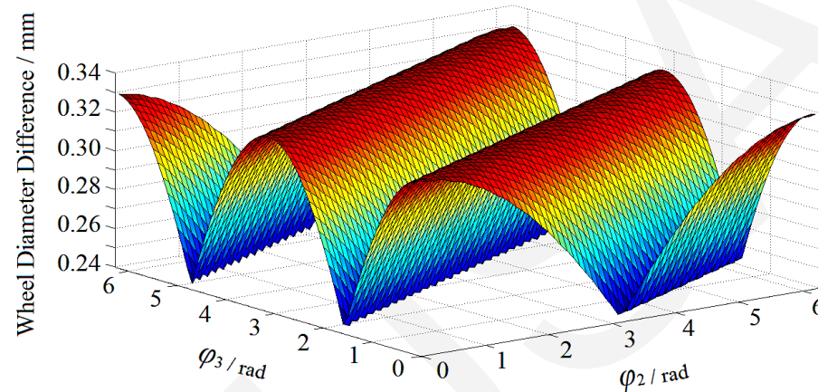
Fig. 16 Wheel diameter differences caused by combination of different phase angles
