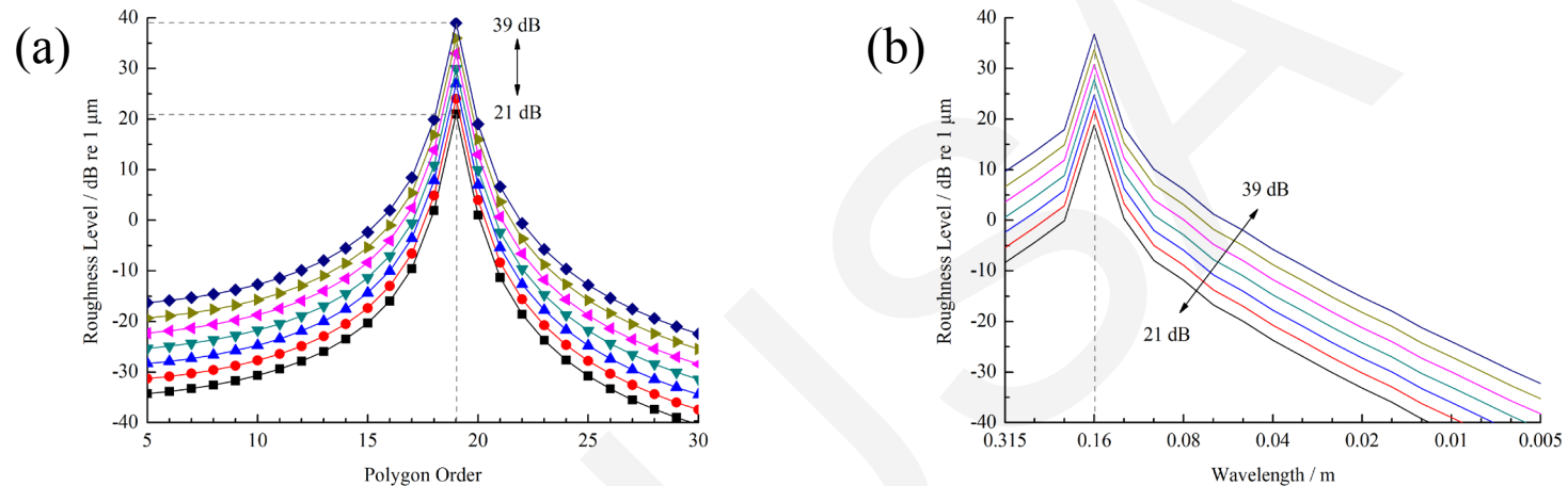
Fig. 14 Different roughness levels: (a) polygon roughness levels characterized by order, (b) polygon roughness levels characterized with the wavelength
