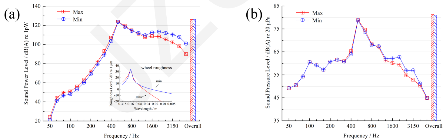
Fig. 17 Different roughness levels: (a) wheel/rail noise, (b) interior noise.
