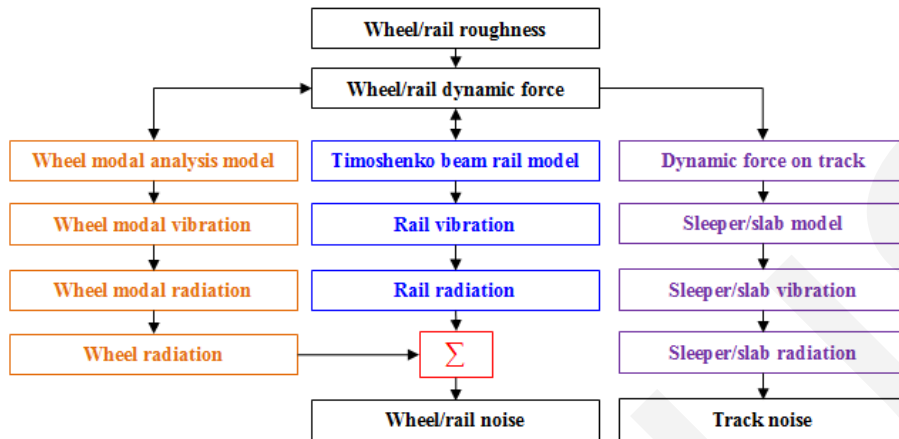
Fig. 6 Wheel/rail noise prediction using the HWTNS (Wu, 2012)
