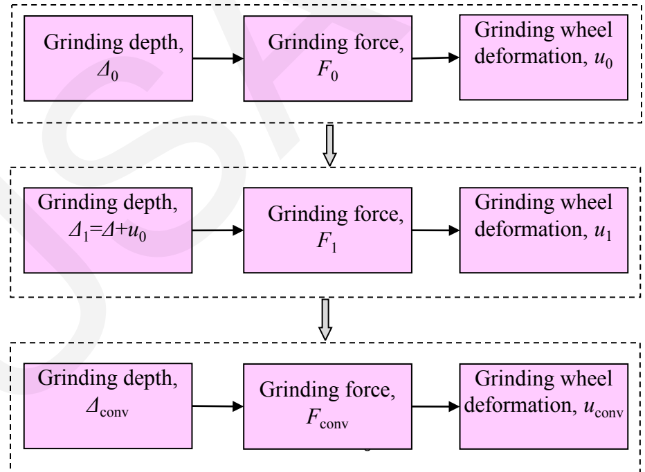
Fig. 6 Coupling iteration process of grinding force and grinding wheel deformation
