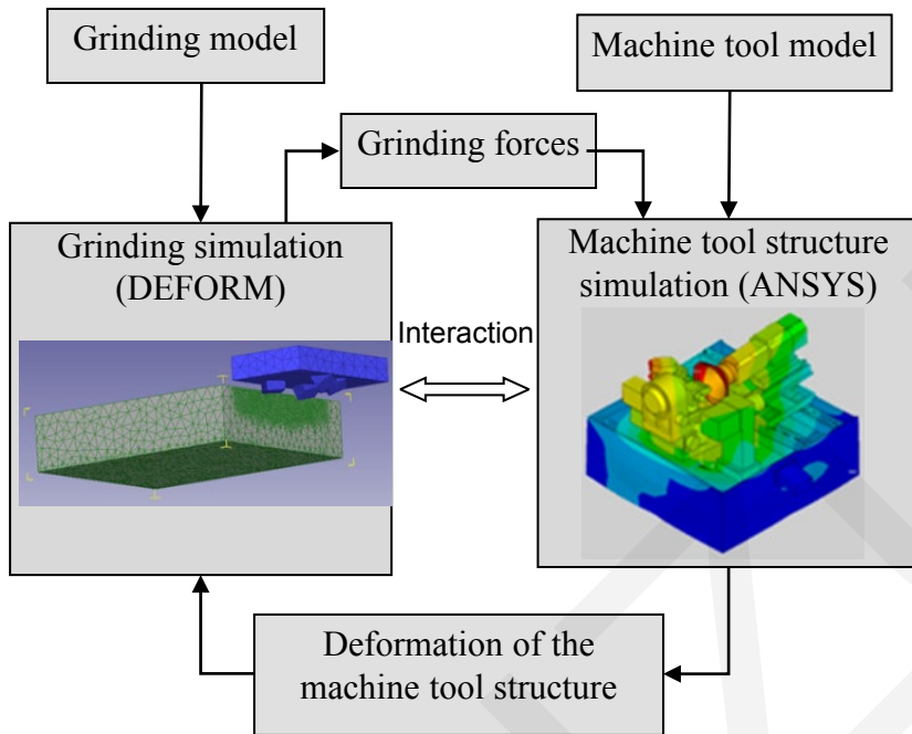
Fig.5 Coupling modeling and simulation of machine-process interaction
