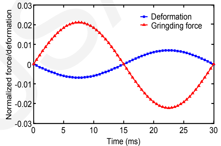
Fig. 8 Coupled iteration of the grinding force and deformation
