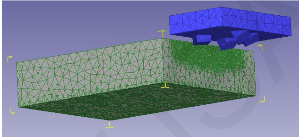
Fig. 4 Finite element model of the virtual grinding wheel and workpiece
