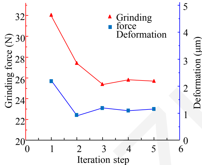
Fig. 7 Iteration of the coupling simulation
