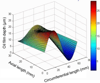
Dynamic oil film depth of piston cylinder pair
