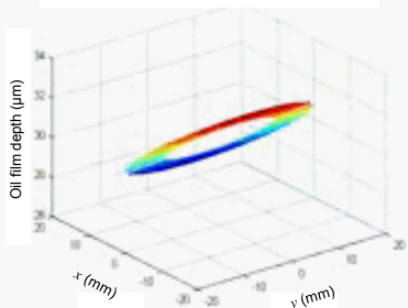
Dynamic oil film depth of slipper swash plate pair
