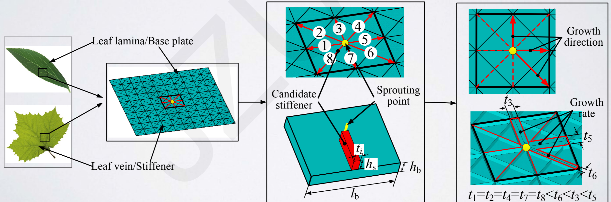
Figure: FE model for growth simulation of plant leaves
