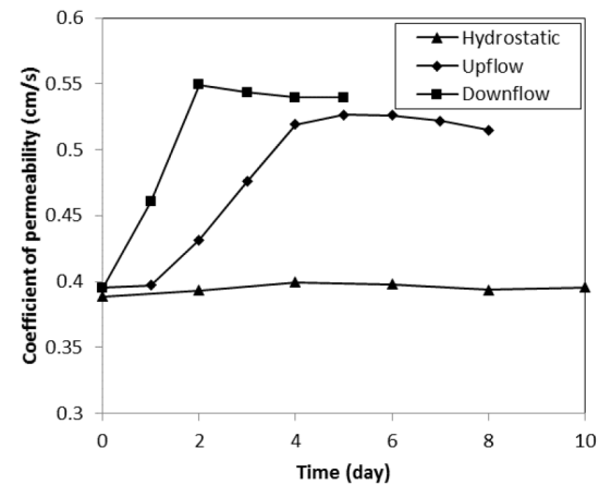
Variation of permeability with time
