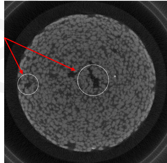
2 - 2' Cross-section
