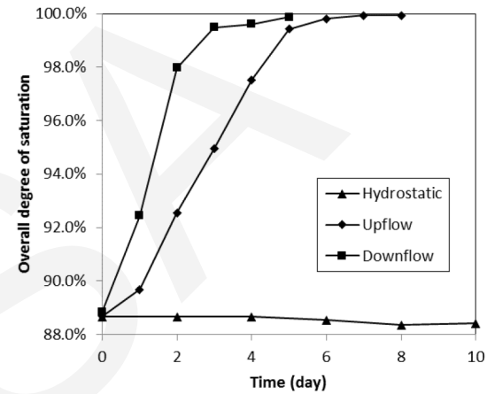
Variation of saturation degree with time
