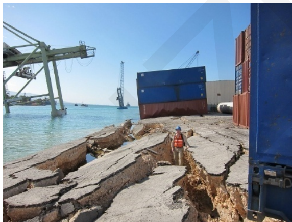
Dislocation of retaining wall (2010 Haiti Earthquake)
