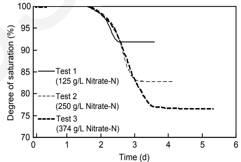
Variation of saturation degree with time in the soil desaturation test
