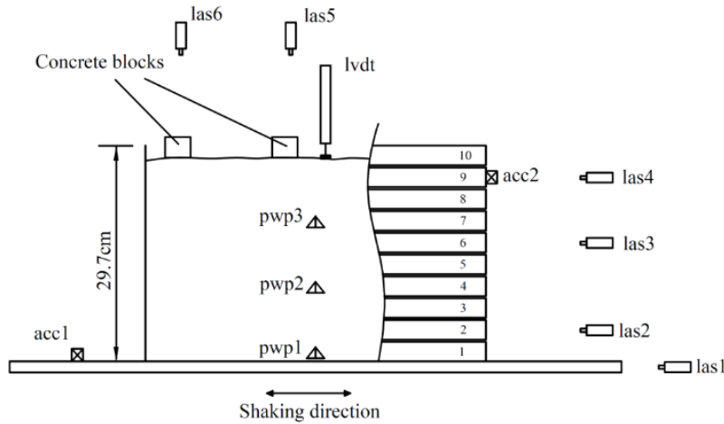
Set-up and instrumentation of shaking table test
