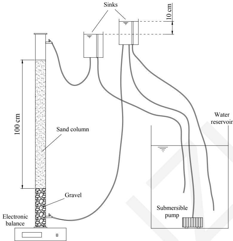
Set-up of gas stability test
