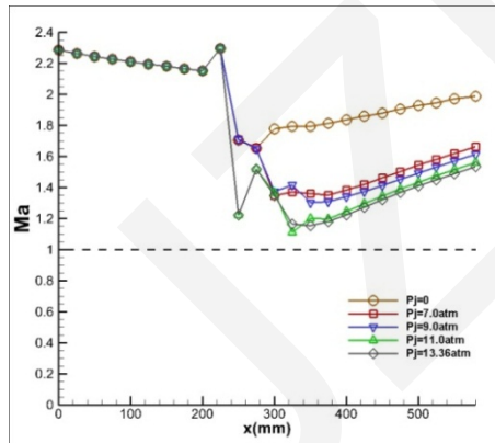
(c) Mass-weighted Mach number
