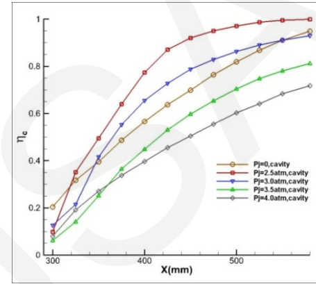
(b) Combustion efficiency
