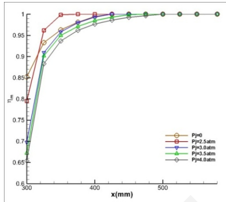
(a) Mixing efficiency
