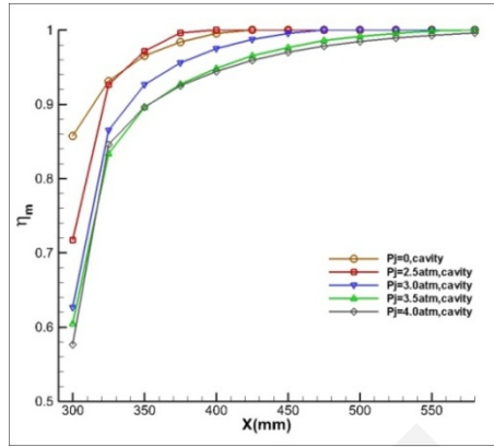
(a) Mixing efficiency
