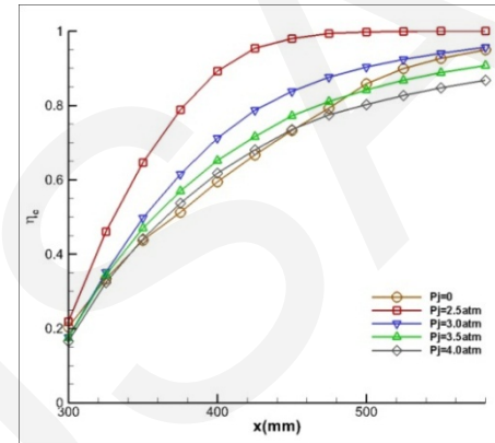
(b) Combustion efficiency
