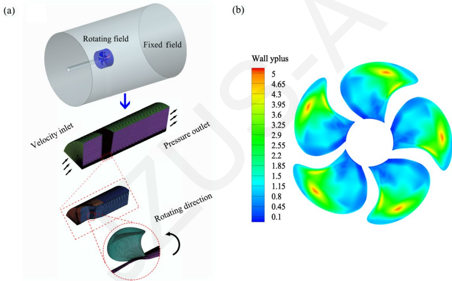
Fig. 1. Calculation domain and grid layout
