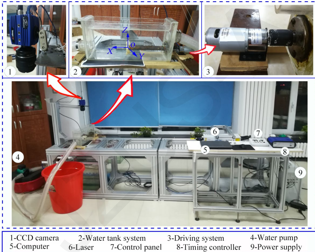
Fig. 3. Basic layout of the PIV system
