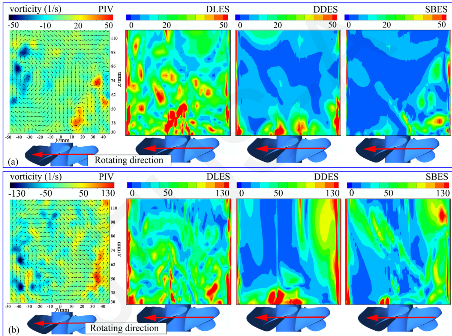
Fig. 4. Instantaneous vorticity field distribution
