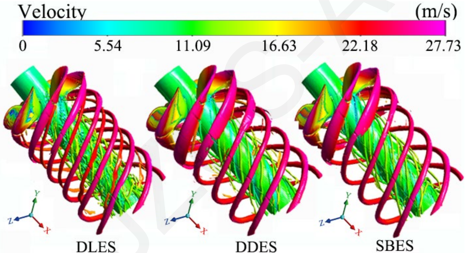
Fig. 2. Vortex distribution behind the propeller
