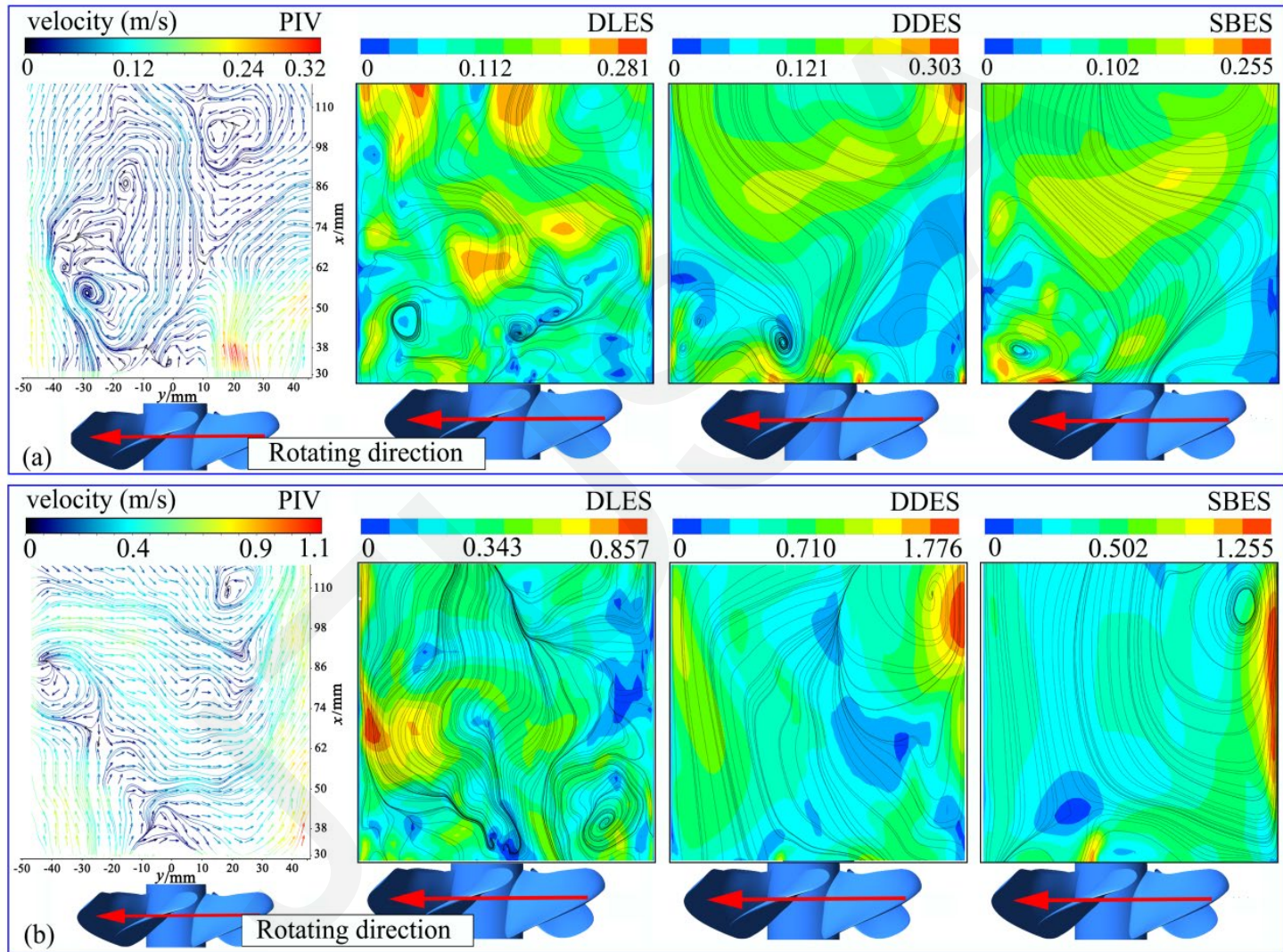
Fig. 5. Instantaneous velocity field distribution
