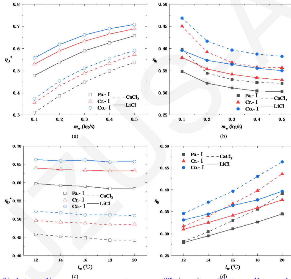
Fig.9 Effects of inlet cooling water parameters on efficiencies of internally-cooled dehumidifiers (a) Effect of m_w on dehumidification efficiency; (b) Effect of m_w on exergy efficiency; (c) Effect of t_w on dehumidification efficiency; (d) Effect of t_w on exergy efficiency
