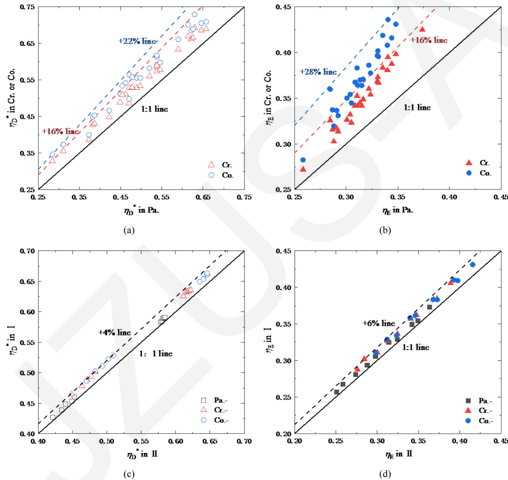
Fig. 4 Effects of flow types on the efficiencies of internally-cooled dehumidifiers
