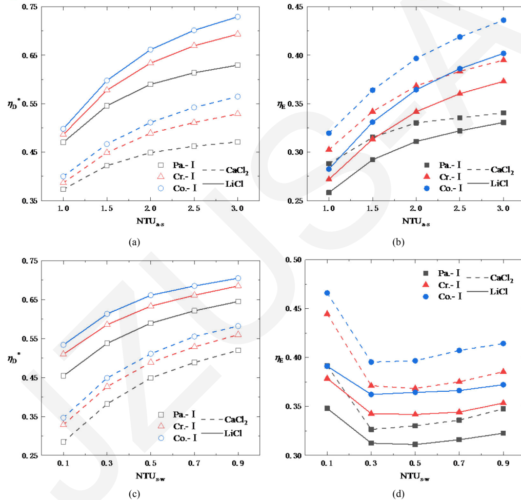
Fig. 5 Effects of NTU on the efficiencies of internally-cooled dehumidifiers
