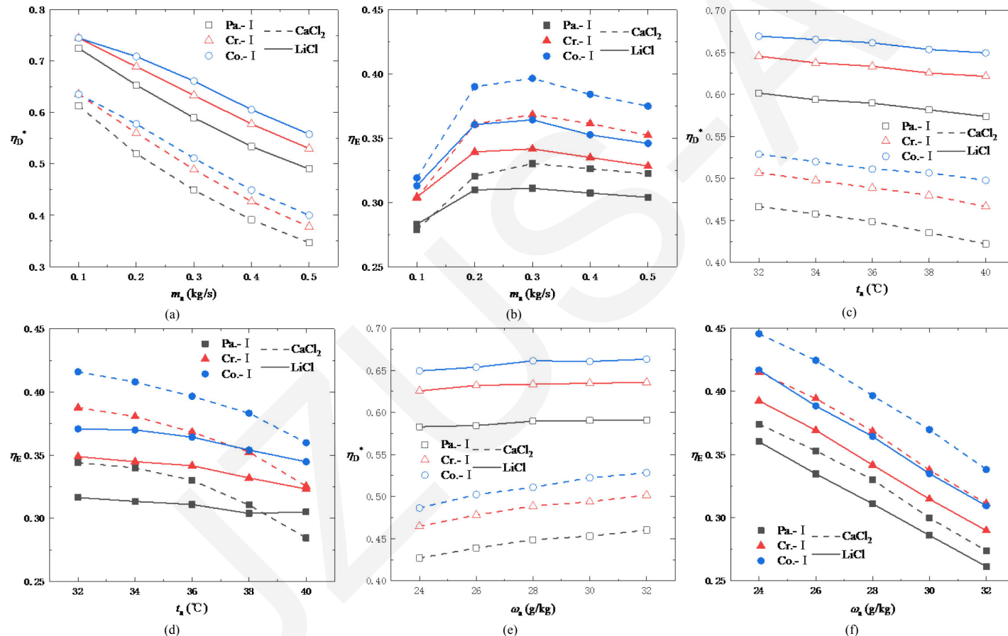
Fig. 8 Effects of inlet air parameters on the efficiencies of internally-cooled dehumidifiers (a) Effect of m_a on dehumidification efficiency; (b) Effect of m_a on exergy efficiency; (c) Effect of t_a on dehumidification efficiency; (d) Effect of t_a on exergy efficiency; (e) Effect of \omega_a on dehumidification efficiency; (f) Effect of \omega_a on exergy efficiency
