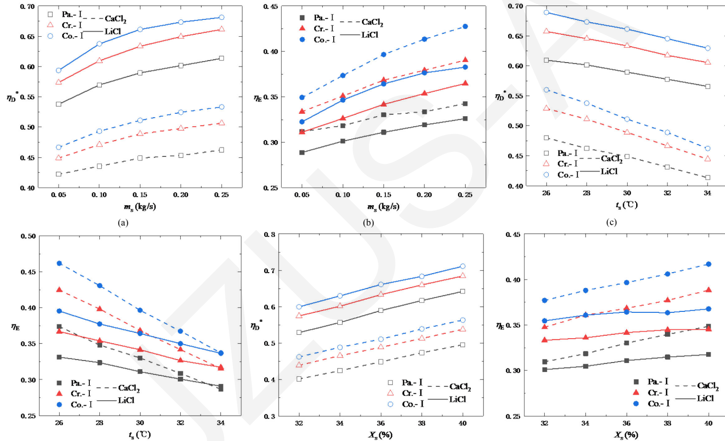
Fig. 7 Effects of inlet solution parameters on the efficiencies of internally-cooled dehumidifiers (a) Effect of m_s on dehumidification efficiency; (b) Effect of m_s on exergy efficiency; (c) Effect of t_s on dehumidification efficiency; (d) Effect of t_s on exergy efficiency; (e) Effect of X_s on dehumidification efficiency; (f) Effect of X_s on exergy efficiency
