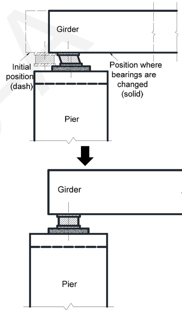
The pre-set distance of bearings
