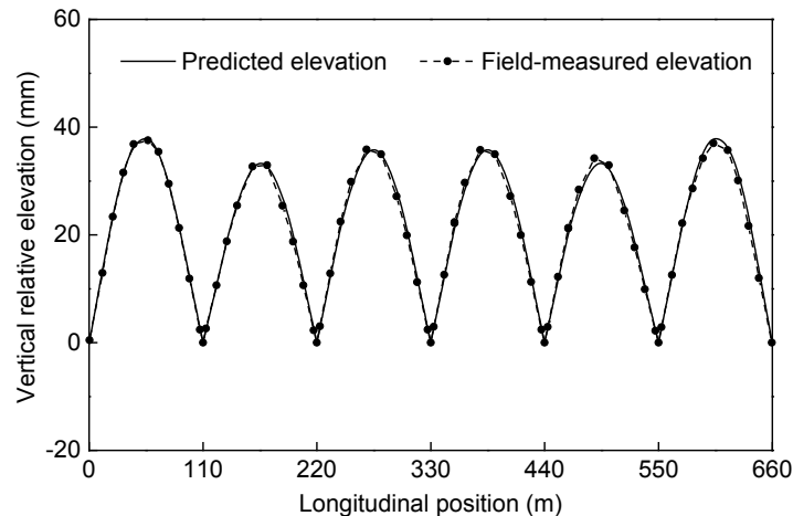
Final vertical relative elevation
