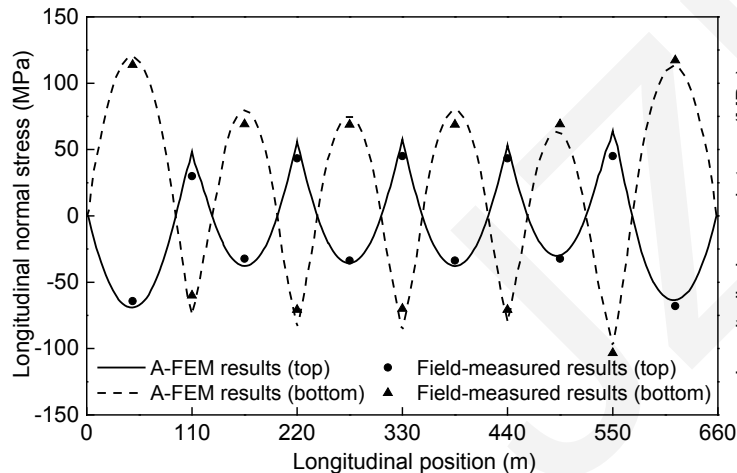
Longitudinal normal stress distribution
