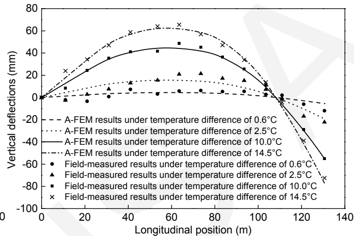
Vertical deflections induced by temperature differences
