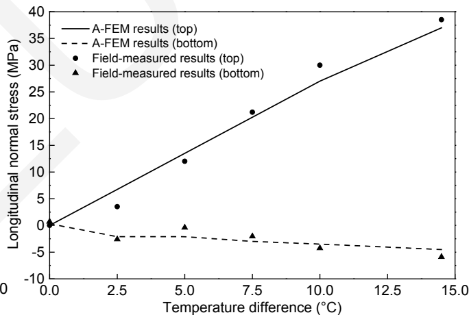
Normal stress at the mid span under different temperature differences
