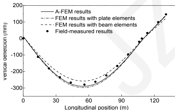
(a) vertical deflections
