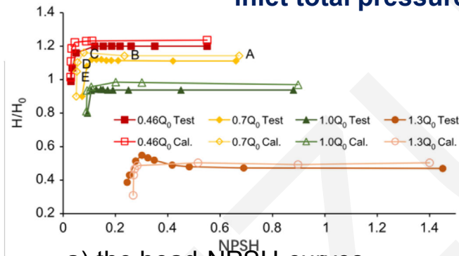
a) the head-NPSH curves
