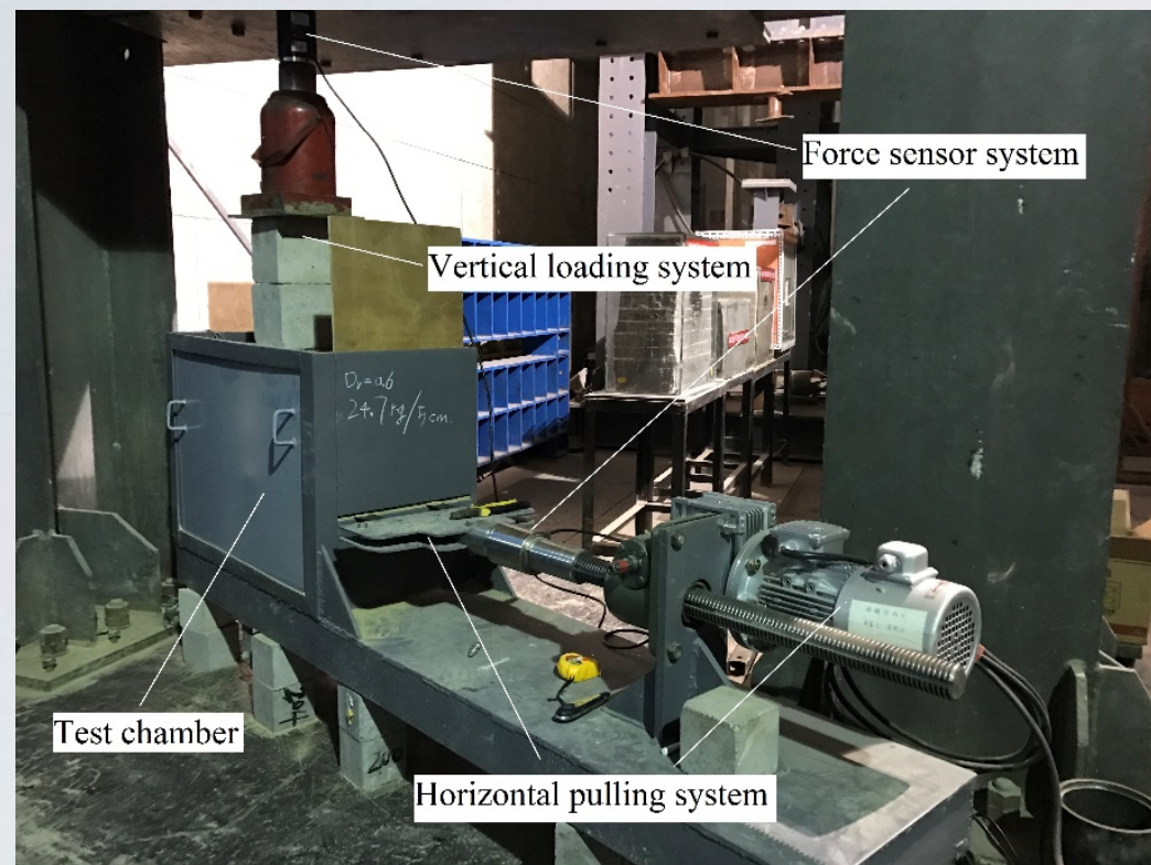
Pullout test device
