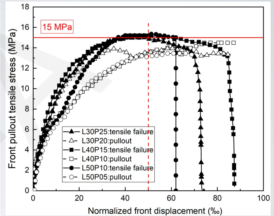
Comparison of two failure cases
