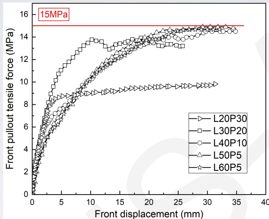
Pullout failure cases
