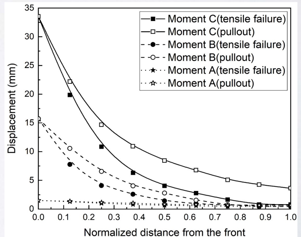
Distributed displacement measurement
