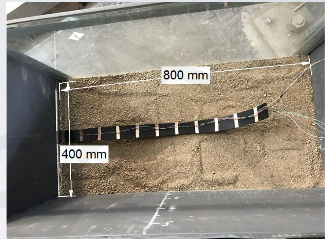
Pullout test preparation
