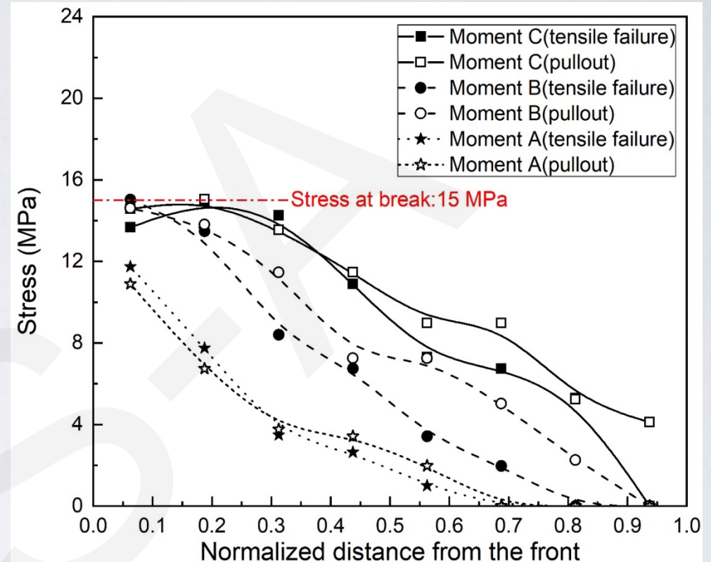
Distributed stress measurement
