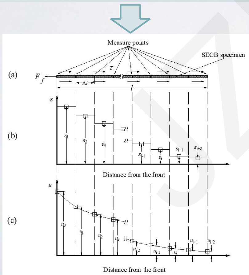
Distributed strain measurement
