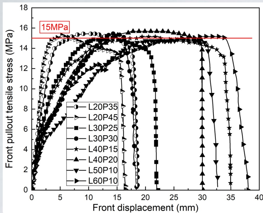
Tensile failure cases
