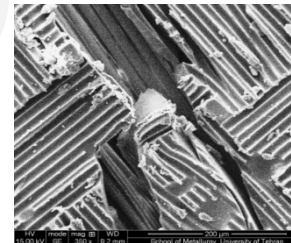
Bridging
