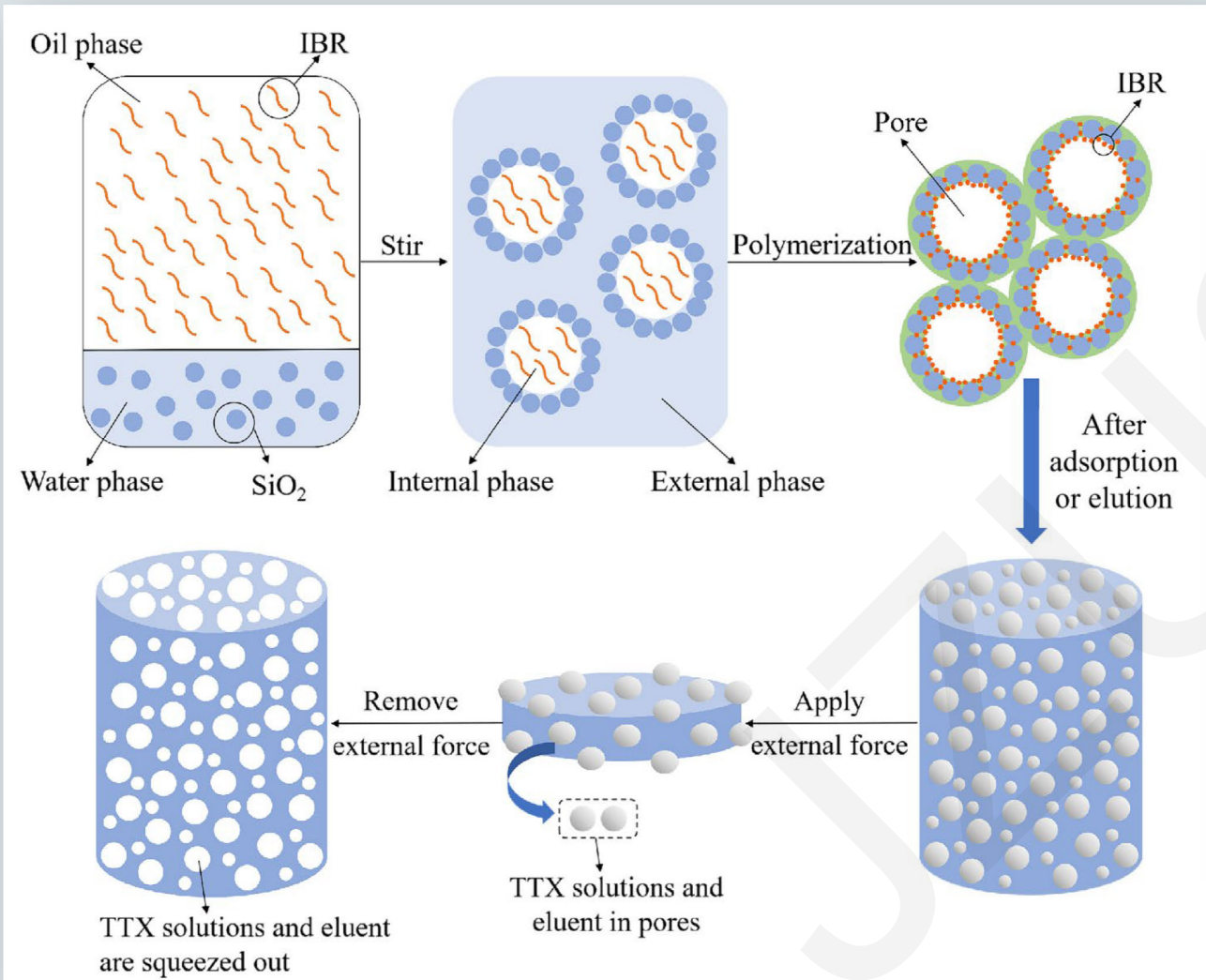
Fig. 1 Formation of \text{SiO}_2@IBR with macroporous structure and good flexibility derived from Pickering O/W HIEPs
