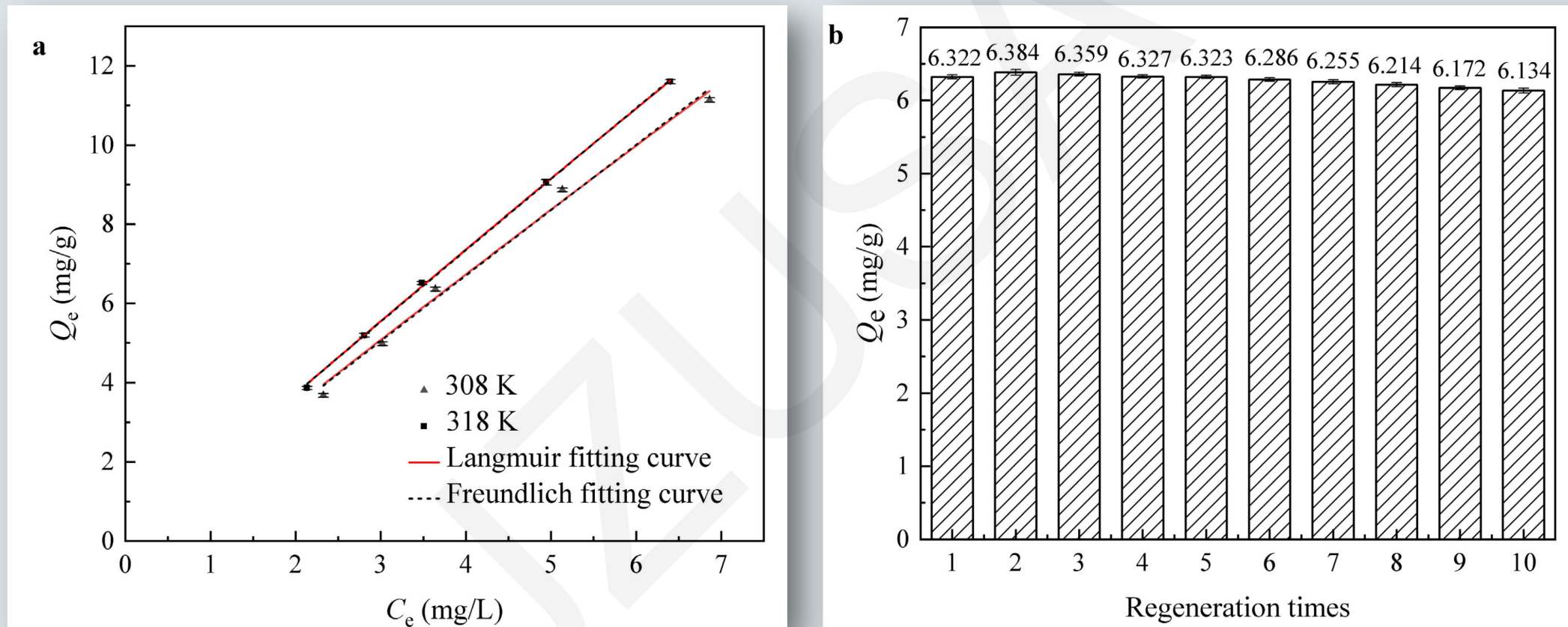
Fig. 6 Equilibrium data and modeling for adsorption of TTX onto \text{SiO}_2@IBR (a) and Regeneration of \text{SiO}_2@IBR for ten cycles (b)
