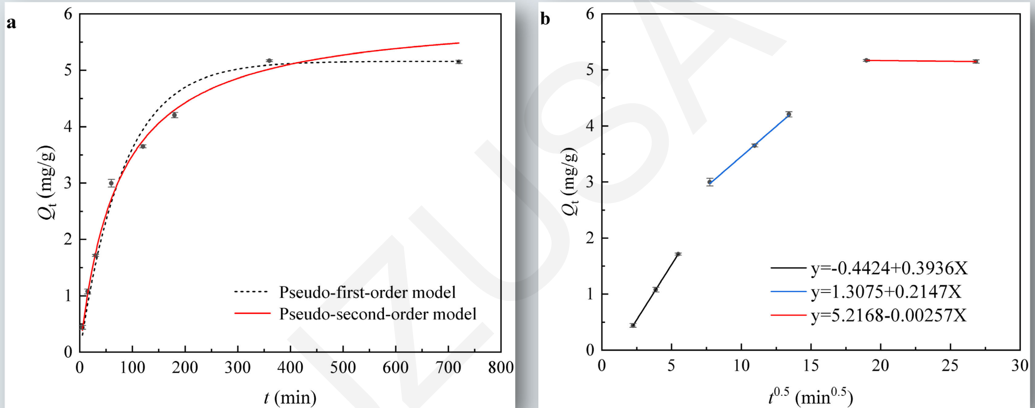
Fig. 5 Kinetic data and modeling for adsorption of TTX onto SiO 2 @IBR (a) and Intra-particle diffusion modeling for adsorption of TTX onto SiO 2 @IBR (b)
