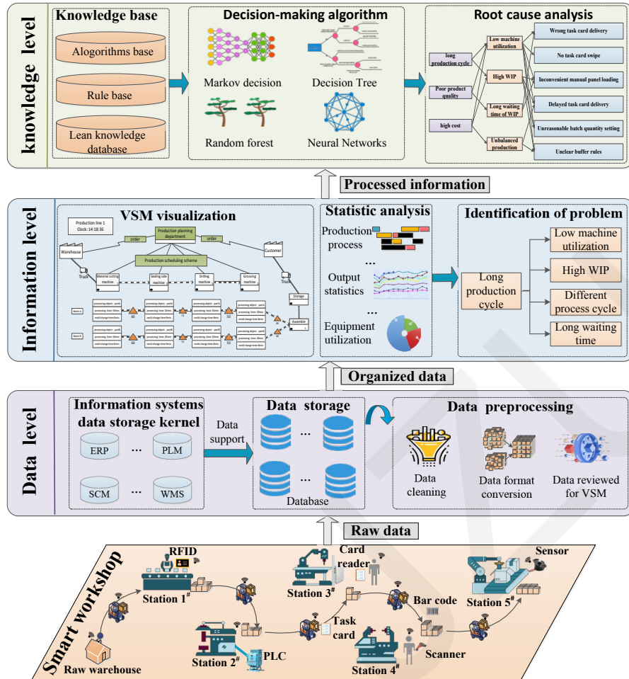
Figure 2. The proposed systematic framework of automated value stream mapping
