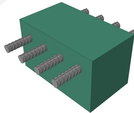
Finite element model
