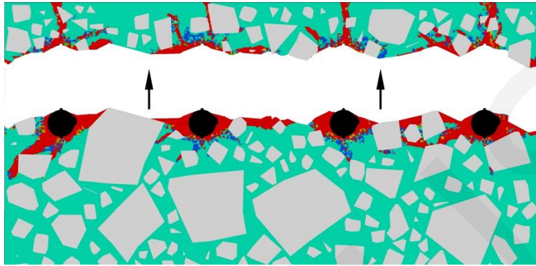
(a) Spalling
