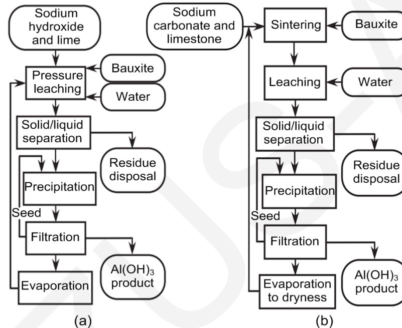
Fig. 1 Production processes of alumina: (a) Bayer process; (b) sintering process.
