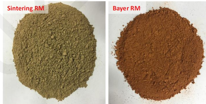
Fig. 2 Morphology of RM produced from sintering and Bayer processes.
