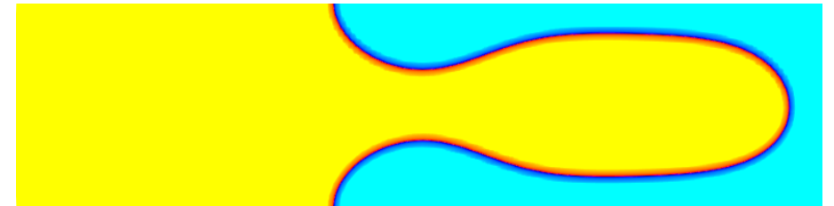
viscous fingering
