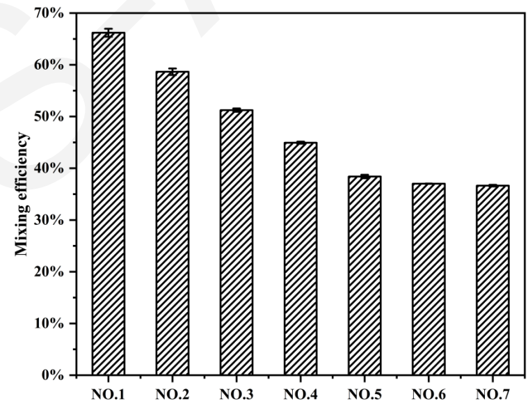
Fig. 2 Dependency of mixing efficiency on the mesh numbers
