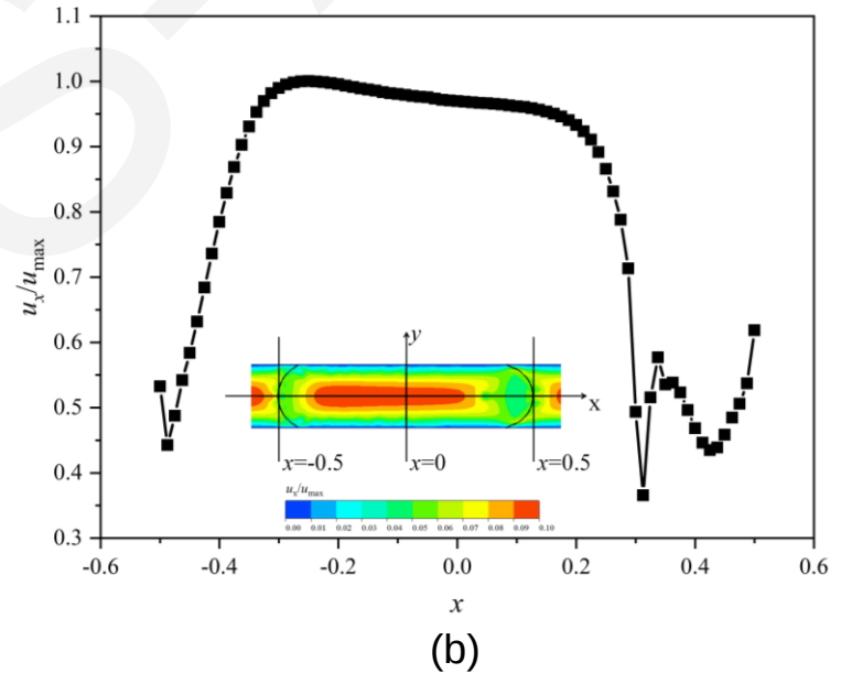
Fig. 7 Velocity gradient in the droplet with u_{\text{sup}}=50 mm/s and \varepsilon_d=0.5 : (a) velocity gradient in the droplet radial direction; (b) velocity gradient in the droplet axial direction
