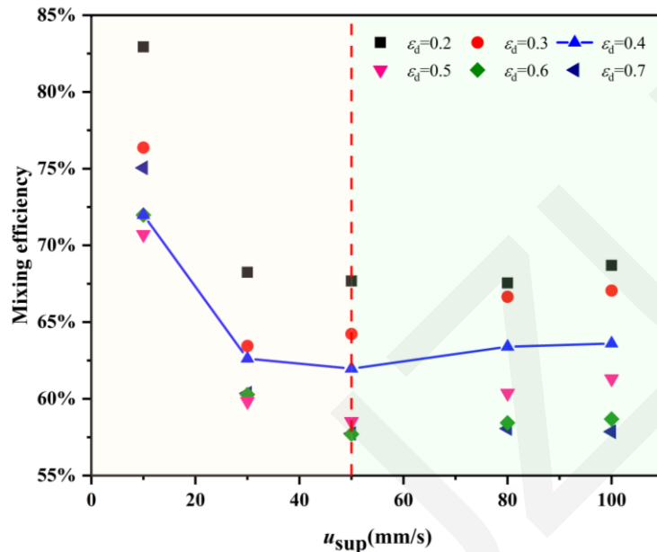
Fig. 10 Mixing efficiency at different droplet superficial velocities at the moment of droplet formation
