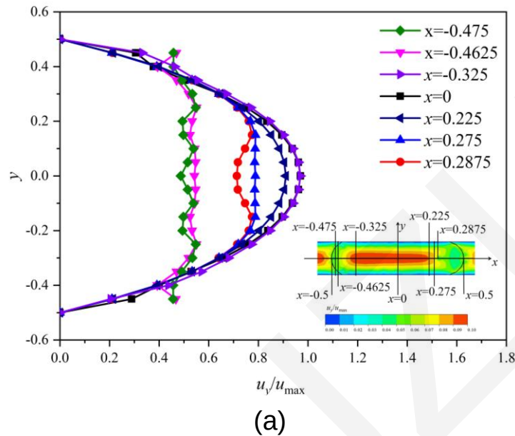
Fig. 7 Velocity gradient in the droplet with u_{\text{sup}}=50 mm/s and \varepsilon_d=0.5 : (a) velocity gradient in the droplet radial direction; (b) velocity gradient in the droplet axial direction
