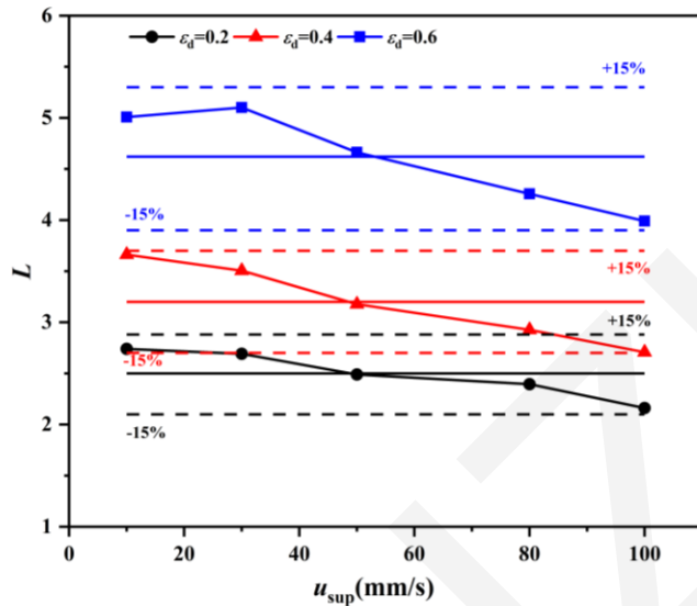
Fig. 5 Variation of the dimensionless droplet length L with different droplet superficial velocities
