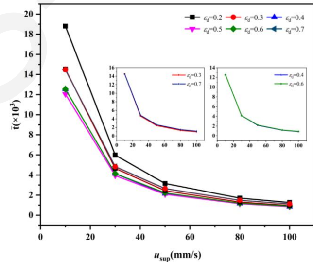
Fig. 6 Variation of dimensionless droplet formation time \bar{t} with different droplet superficial velocities
