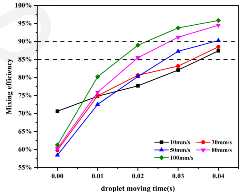
Fig. 11 Mixing efficiency at different droplet superficial velocities in the droplet moving stage with \epsilon_d=0.5
