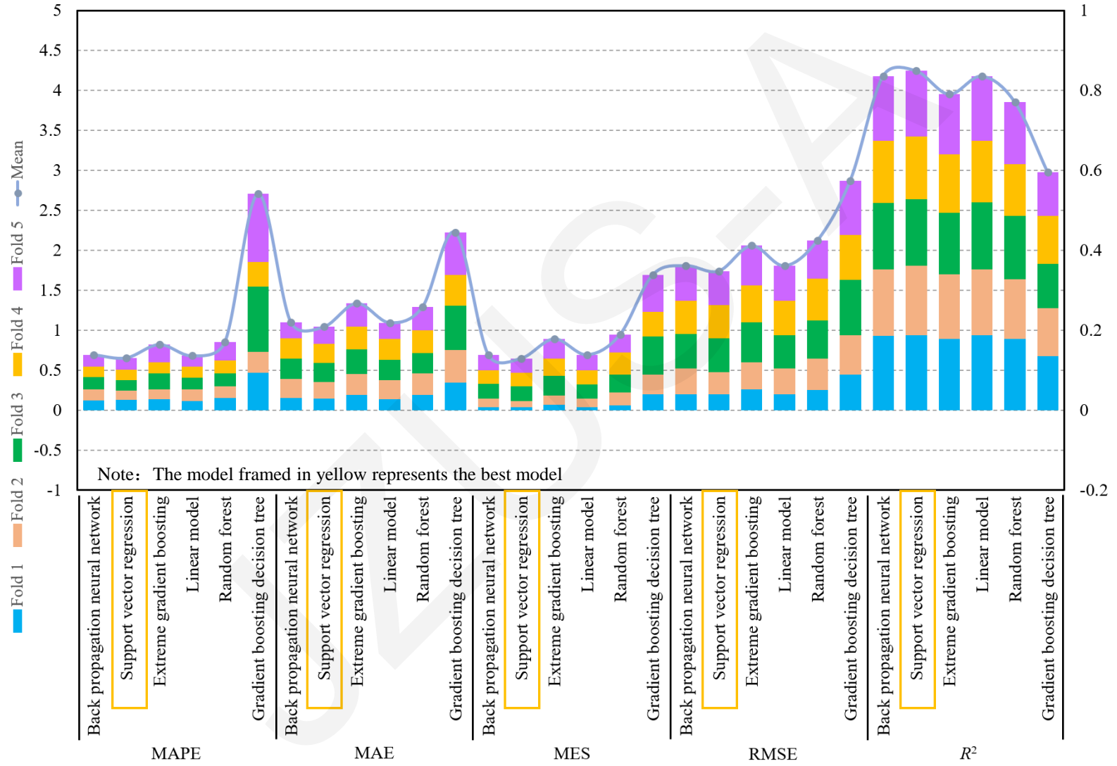
Prediction performance of different single ML models as meta-learner
