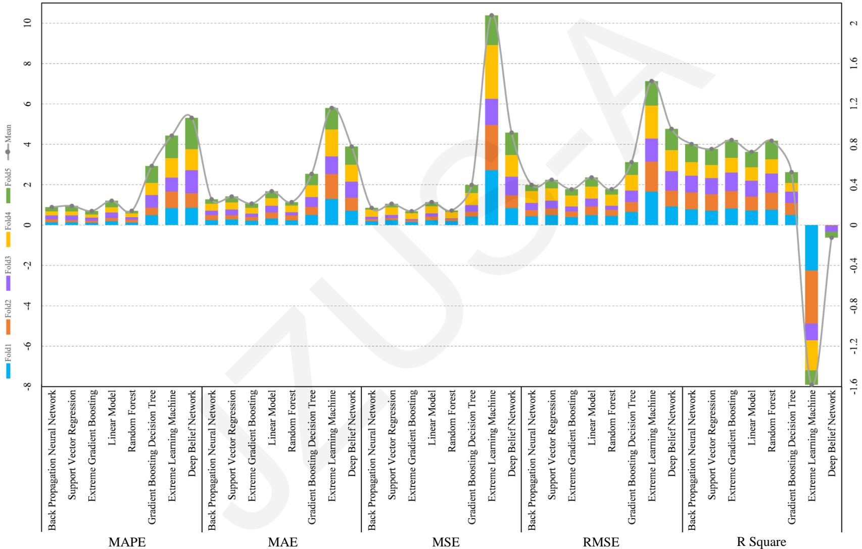
Prediction performance of eight single ML models for base learner
