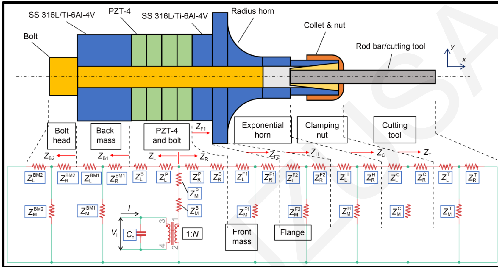
Fig. 5 Equivalent circuit model with T-type equivalent impedance structure
