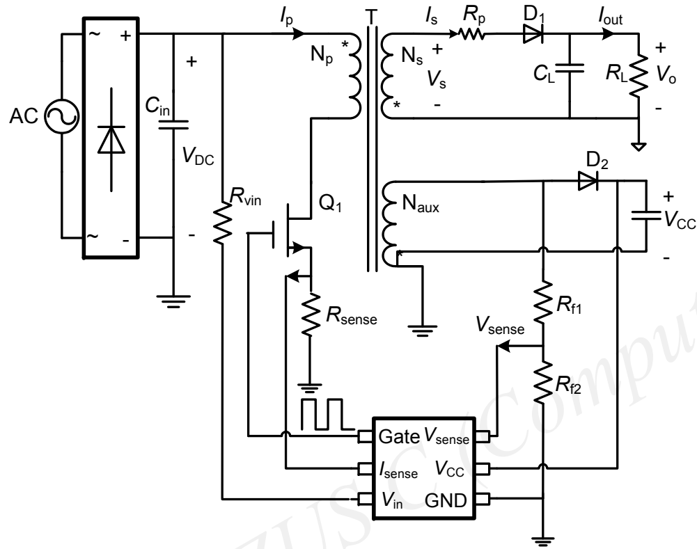
Primary-side feedback flyback with the proposed digital controller
