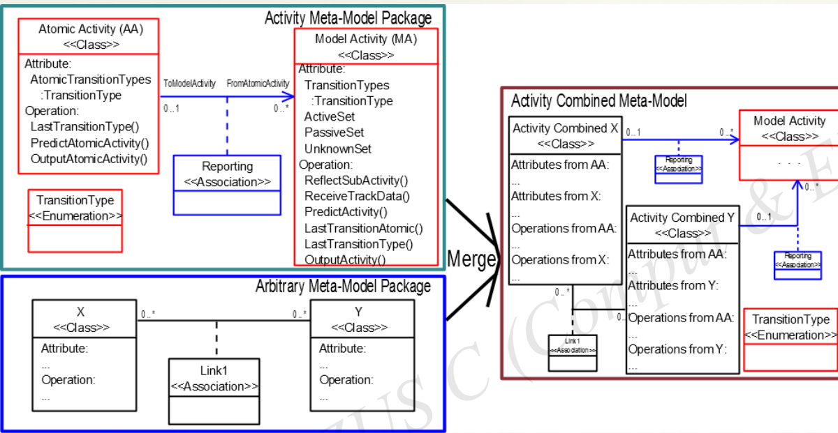
Fig. 6 Integrating activity meta-model into an arbitrary meta-model
