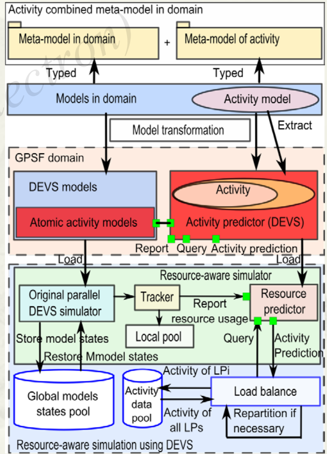
Fig. 9 Framework of resource-aware simulation
