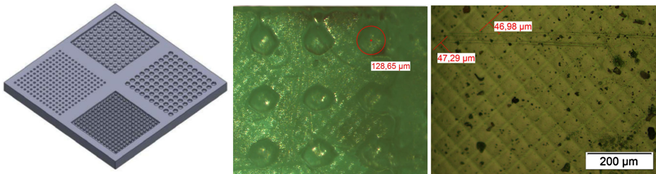
Fig. 1 Micro-features by DLP part (total part size 7 \times 7 \times 0.5 mm). Pixilation structure due to resolution of DLP. Courtesy University of Las Palmas de Gran Canaria
