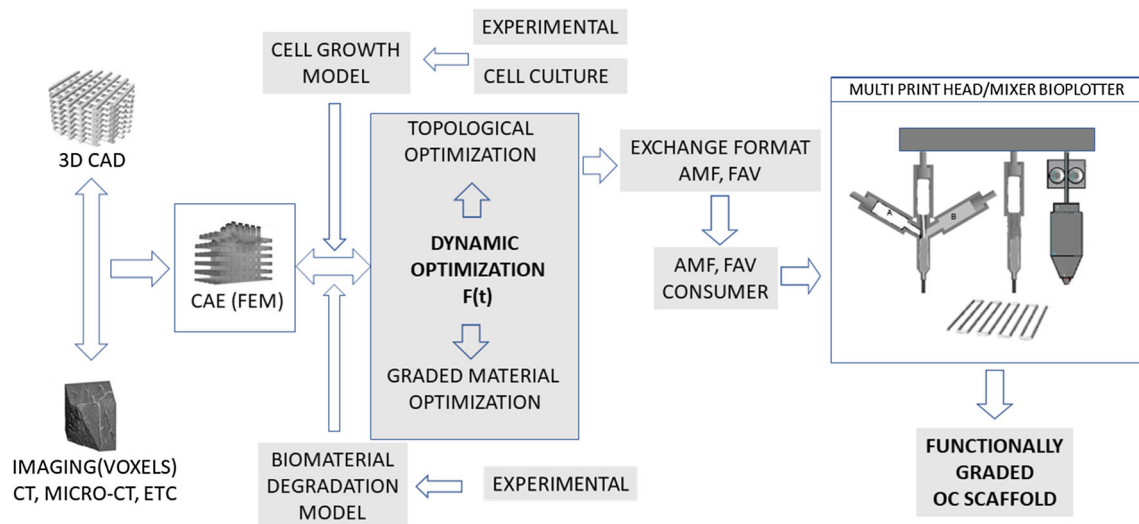
Fig. 5 General methodology for design and manufacturing Functionally Graded OC scaffolds
