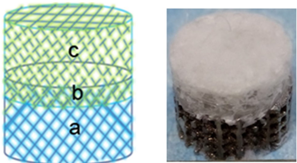
Fig. 3 Gradient structure. a Titanium matrix b PLA junction c PLGA infiltrated collagen layer. Courtesy University College London
