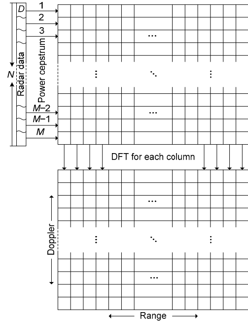
Fig. 4 Signal flow diagram of the detection algorithm
