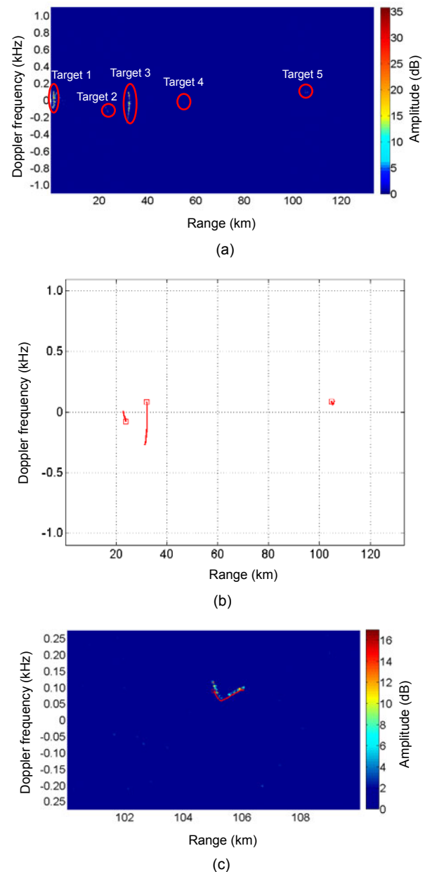
Fig. 10 Target tracks of multiple moving targets
