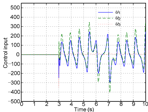
Fig. 2 Control inputs
