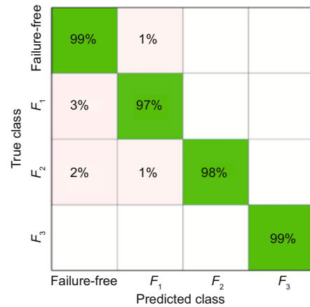
Fig. 12 Confusion matrix corresponding to cubic SVM
