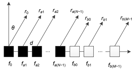
Fig. 6 Single-sided subarray-based frequency diverse array (SB-FDA)
