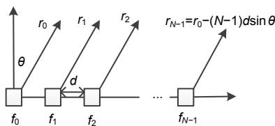
Fig. 1 Basic uniform linear array frequency diverse array (ULA-FDA)
