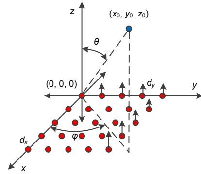
Fig. 4 Planar frequency diverse array (PFDA)
