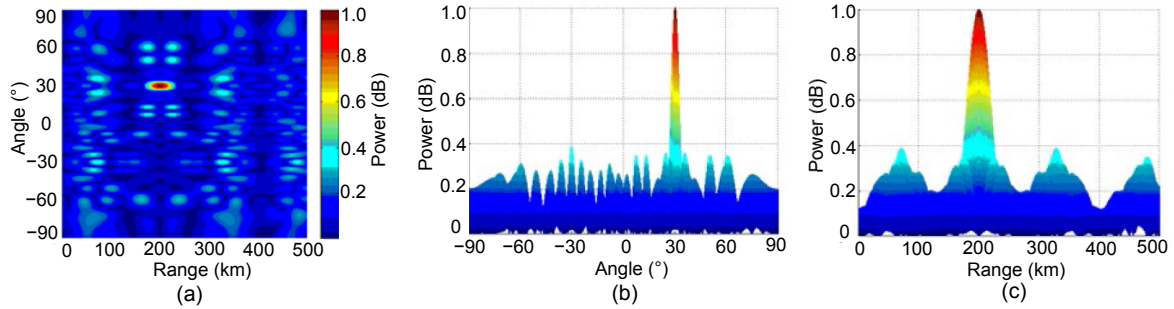
Fig. 23 Transmit beampattern of the centrosymmetric SB-FDA when N=30 , \Delta f=3 kHz, and L=3 : (a) top view; (b) left view; (c) front view
