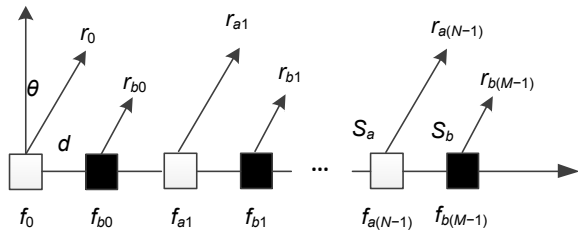
Fig. 9 Cross subarray-based frequency diverse array (SB-FDA)
