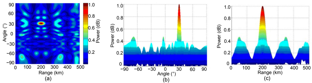
Fig. 24 Transmit beampattern of the centrosymmetric SB-FDA when N=20 , \Delta f=2 kHz, and L=5 : (a) top view; (b) left view; (c) front view
