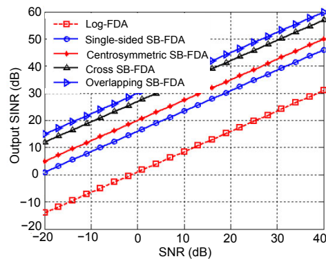
Fig. 20 Performance comparison of the SINR of different FDA radars
