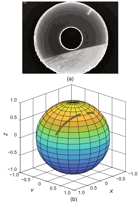
Fig. 12 Sun-pointing mode: (a) raw image; (b) circle E without noisy points
