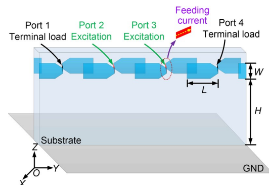
Fig. 1 Schematic of the dipole array with arms overlapped
