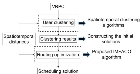
Fig. 4 Integrated framework of the spatiotemporal distance embedded hybrid ant colony algorithm
