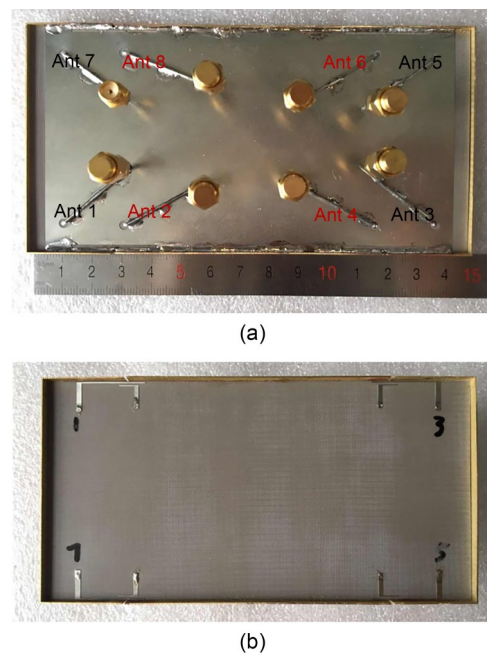
Fig. 10 Fabricated eight-element MIMO array: (a) top view; (b) bottom view
