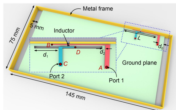
Fig. 1 Structure of the compact building block ( L=28.1 \text{ mm} , d_0=2.50 \text{ mm} , d_1=10.15 \text{ mm} , d_2=2.05 \text{ mm} )
