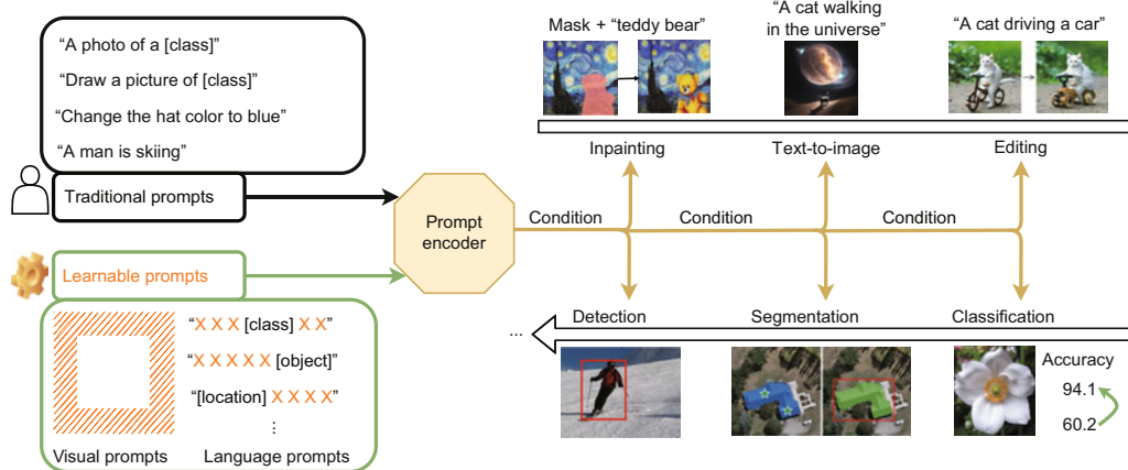
Fig. 1 Pipeline of learning with traditional and learnable prompts. Prompt learning is a critical technique in current AIGC tasks. Apart from human-understandable prompts, learnable prompts have been proposed to further enhance specific tasks
