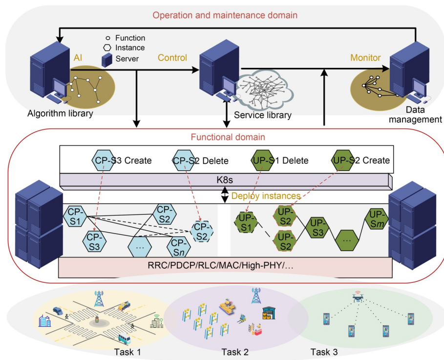
Fig. 1 Dynamic service-based RAN (RAN: radio access network; CP: control plane; AI: artificial intelligence; UP: user plane; RRC: radio resource control; PDPC: packet data convergence protocol; RLC: radio link control; MAC: media access control; PHY: physical)
