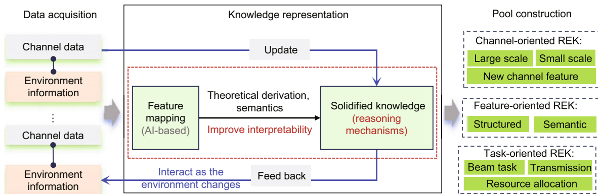
Fig. 2 REKP architecture with its core function being the construction of REK (REK: radio environment knowledge; REKP: REK pool)
