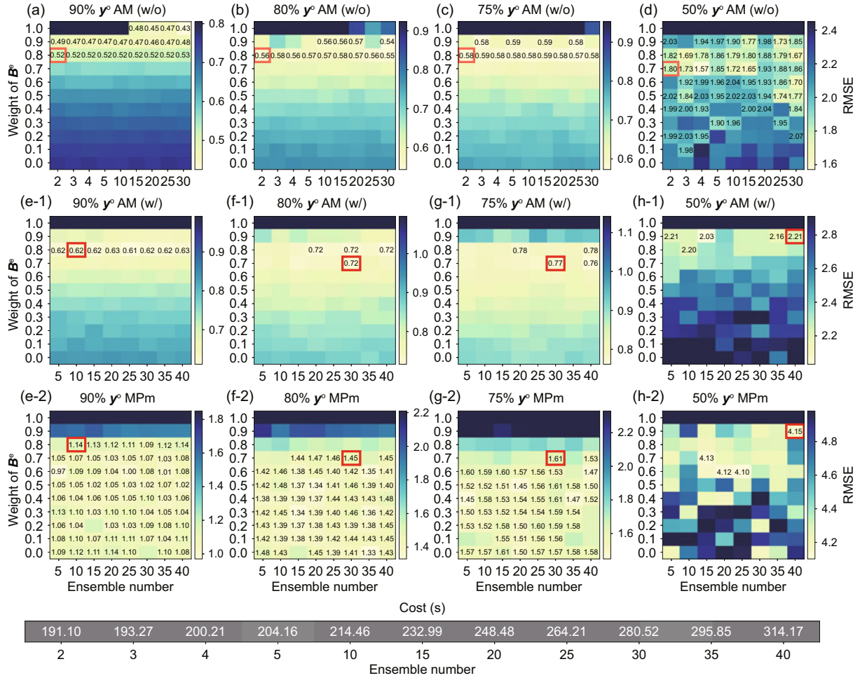
Fig. 4 HCDA assimilation performance heatmaps. Results are shown from left to right for 90% y^\circ , 80% y^\circ , 75% y^\circ , and 50% y^\circ . The gray heatmap represents the computational cost. Figs. 4a–4d correspond to Experiment 1 (without mutation), and Figs. 4e–4h correspond to Experiment 2 (with mutation). Index 1 represents the AM RMSE (line 2), and index 2 represents the RMSE during the mutation period (MPm) (line 3). References to color refer to the online version of this figure
