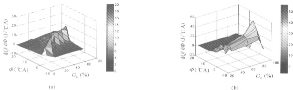
Fig.6 Effect of natural gas quantity on combustion rate (a) at light load (b) at heavy load
