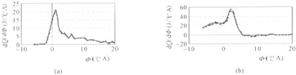
Fig.3 Comparison of simulated result of combustion rate with test data (a) light load condition (b) heavy load condition
