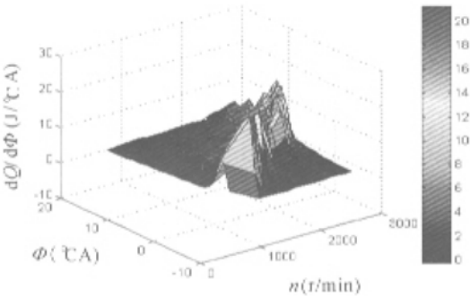
Fig.4 Effect of rotative speed on combustion rate
