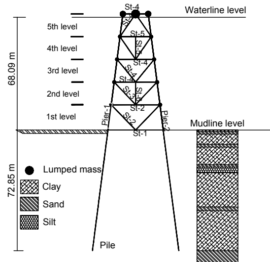
Fig. 10 Soil profile and other specifications
