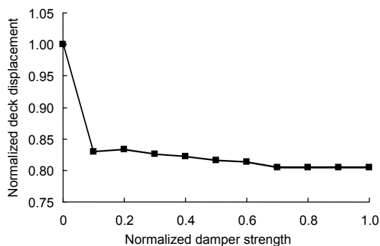
Fig. 26 Normalized deck displacement of jacket vs. normalized strength of damper for Sylmar record
