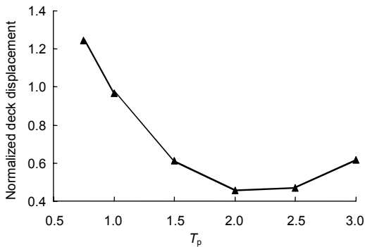
Fig. 21 Normalized responses of jacket vs. period of equivalent pulse of near-fault earthquake (PGA=6 m/s 2 )
