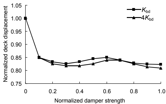
Fig. 24 Normalized deck displacement of jacket vs. normalized strength of damper for ICC000 record (PGA = 8.25 m/s 2 )
