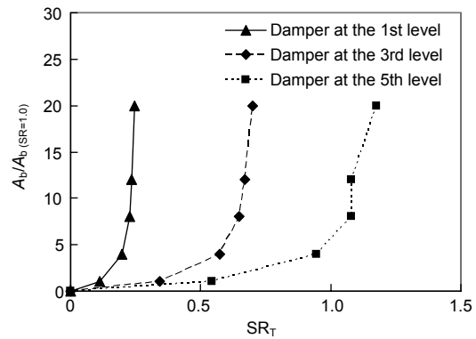
Fig. 16 Stiffness ratio of the total structure vs. brace area
