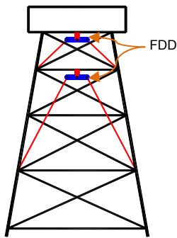
Fig. 5 Jacket platform retrofitted with FDD
