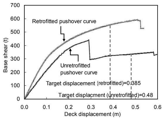
Fig. 17 Pushover curve of the jacket for retrofitted and unretrofitted cases
