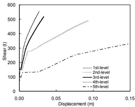
Fig. 18 Pushover curve of each level for retrofitted case
