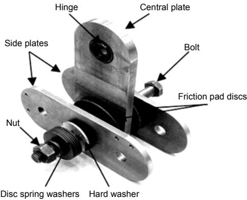
Fig. 4 Components of FDD (Mualla and Nielsen, 2002)
