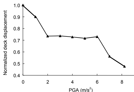
Fig. 28 Normalized deck displacement of jacket vs. PGA of Sylmar record
