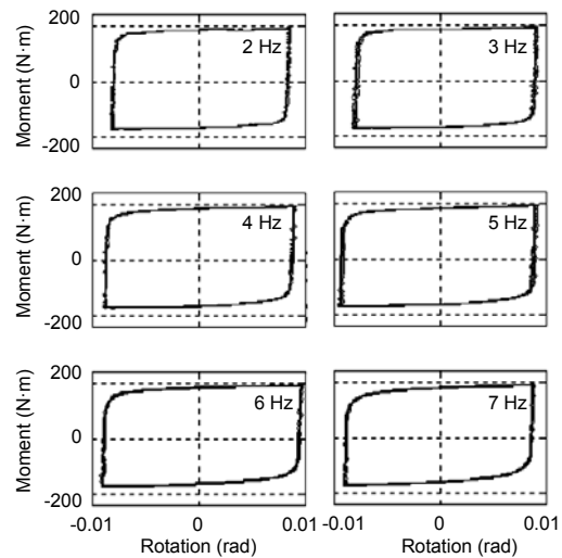
Fig. 6 Effect of forcing frequency on hysteretic loop (Mualla and Belev, 2002)
