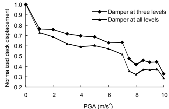
Fig. 27 Normalized deck displacement of jacket vs. PGA of CHY101W record
