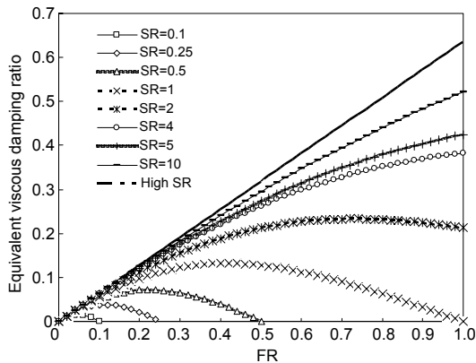
Fig. 8 Equivalent viscous damping ratio for dual system (Tabeshpour and Ebrahimiyan, 2010)
