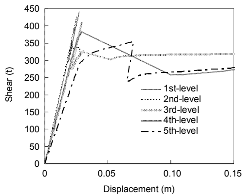
Fig. 15 Pushover of each level of the platform
