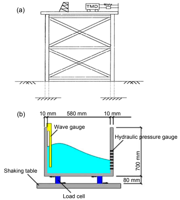
Fig. 3 Control systems for jacket platform structures (a) Tuned mass damper; (b) Tuned liquid damper
