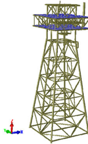
Fig. 9 Perspective plot of Resselat service platform
