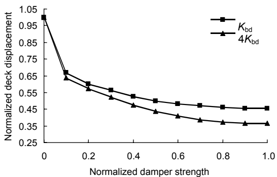
Fig. 25 Normalized deck displacement of jacket vs. normalized strength of damper for CHY101W record (PGA = 7.6 m/s 2 )
