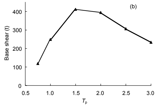
Fig. 20 Responses of jacket vs. period of equivalent pulse of near-fault earthquake (PGA=1 m/s 2 )
