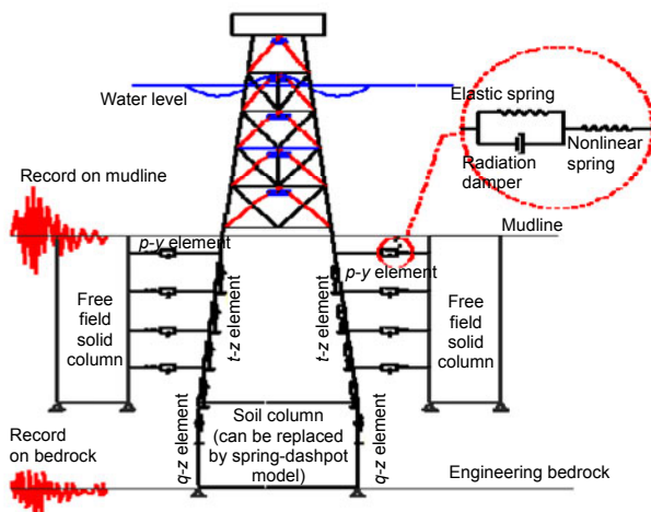
Fig. 12 Modeling of pile-soil-structure interaction
