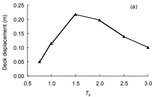
Fig. 20 Responses of jacket vs. period of equivalent pulse of near-fault earthquake (PGA=1 m/s 2 )
