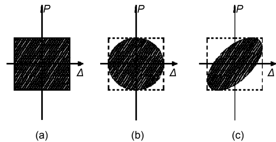
Fig. 7 Comparison of hysteresis loops of different dampers
