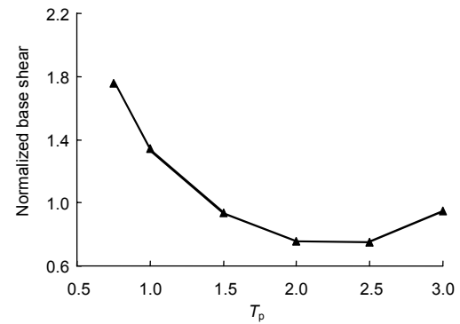
Fig. 21 Normalized responses of jacket vs. period of equivalent pulse of near-fault earthquake (PGA=6 m/s 2 )
