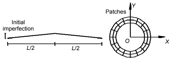
Fig. 11 Modeling of strut and portal members
