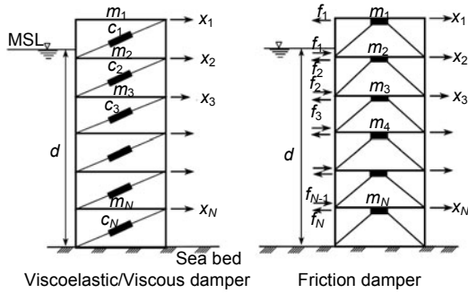
Fig. 1 Viscoelastic, viscous and friction dampers for jacket offshore platforms (Patil and Jangid, 2005) MSL and d are the mean sea level and depth, respectively; m_i , c_i , and f_i are the mass, damping ratio of damper, and restoring force at the i th ( i=1,2,\dots,N ) level, respectively
