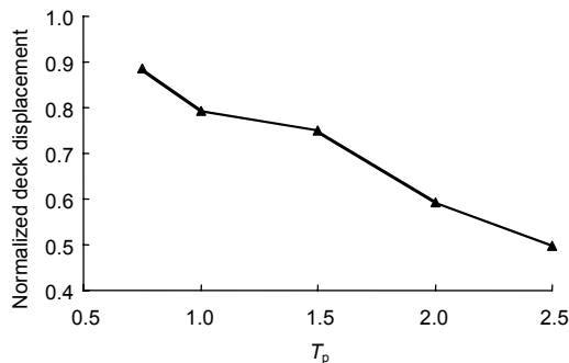
Fig. 22 Normalized deck displacement of jacket vs. period of equivalent pulse of near-fault earthquake (PGA=6 m/s 2 )
