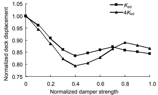
Fig. 23 Normalized deck displacement of jacket vs. normalized strength of damper for ELC-NS record (PGA=3.4 m/s 2 )
