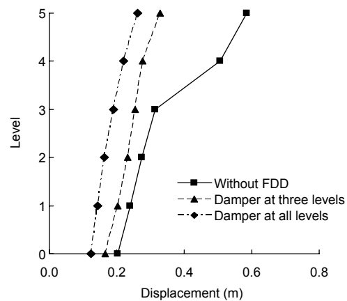
Fig. 19 Displacement of each level of jacket vs. heights
