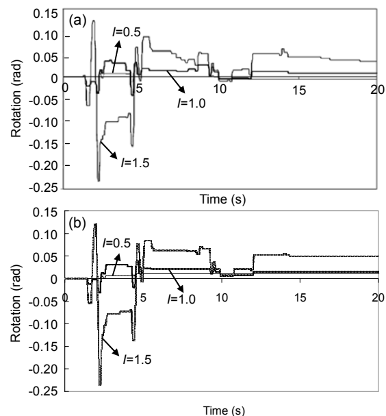
Fig. 14 Effect of ground motions on damper performance (a) Mualla and Belev (2002); (b) OpenSees model. I is the scale factor imposed to the ground motion
