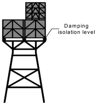
Fig. 2 Offshore jacket platform installed with damping isolation system (Ou et al., 2007)
