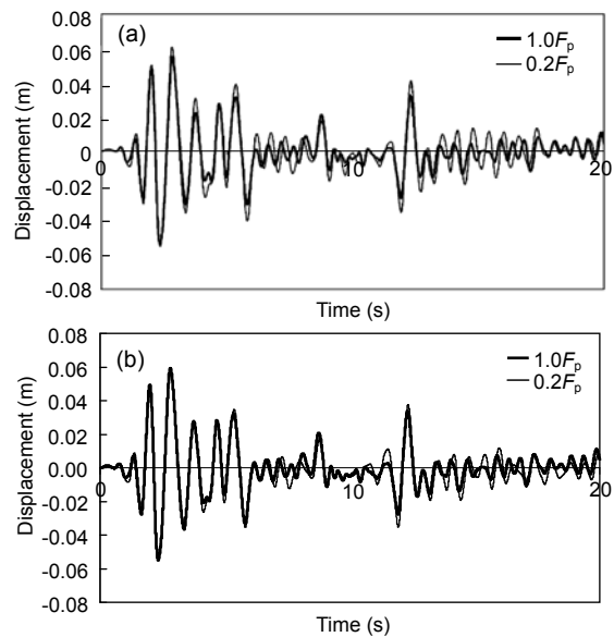
Fig. 13 Effect of pretension force ( F_p ) of damper bars on displacement response (a) Mualla and Belev (2002); (b) OpenSees model
