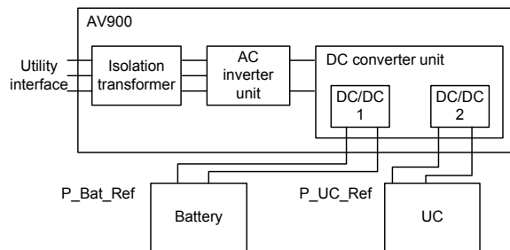
Fig. 22 Topology of HESS test
