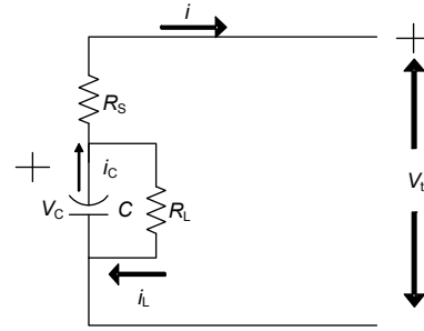
Fig. 4 Ultra-capacitor model
