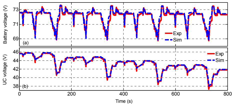
Fig. 24 Voltage of battery/UC under ECE driving cycle
