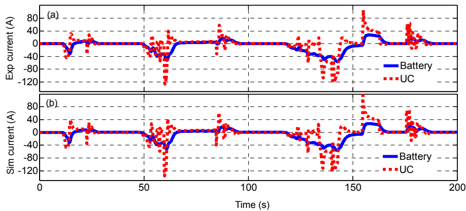
Fig. 23 Current of battery/UC under ECE driving cycle
