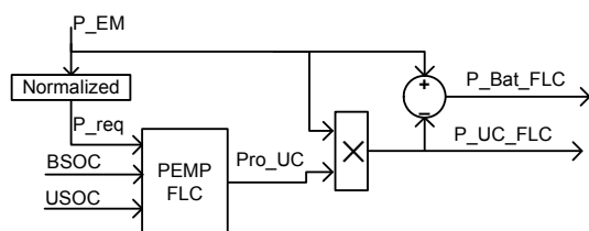
Fig. 10 Block diagram of PEMP FLC
