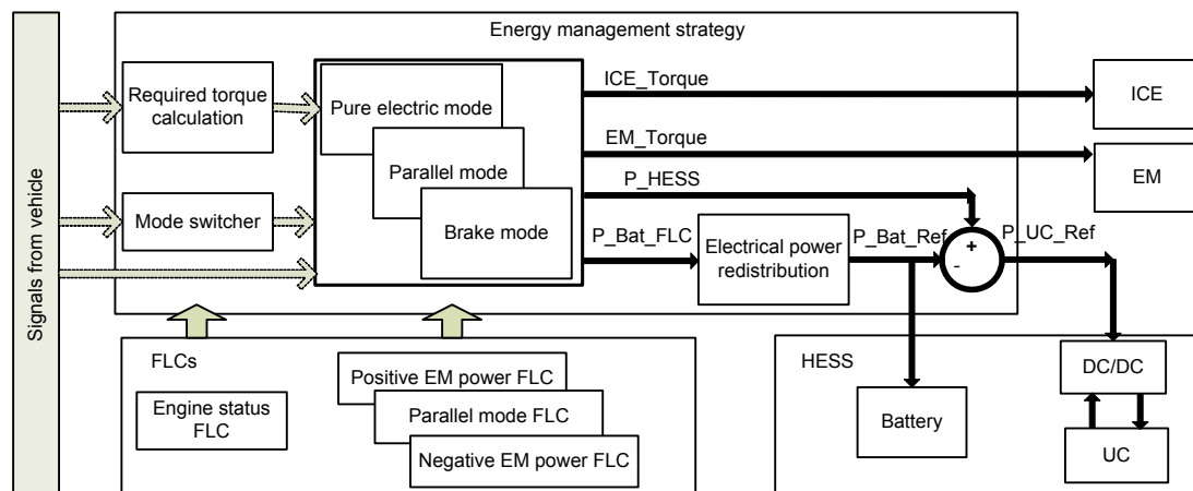
Fig. 5 EMS topology
