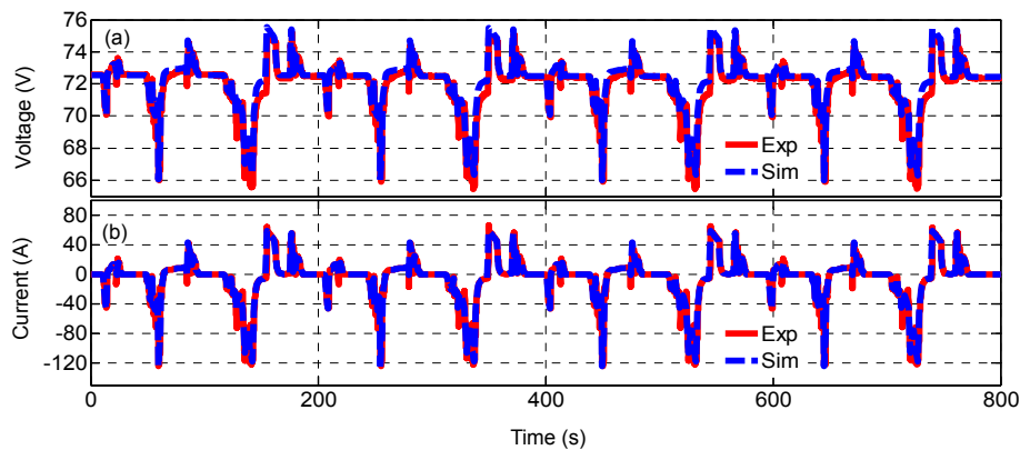
Fig. 25 Voltage and current of battery only system under ECE driving cycle
