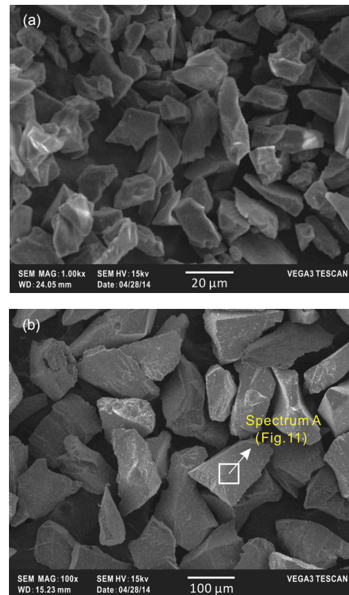
Fig. 2 Typical SEM micrographs of different abrasives (a) 25 \mu\text{m} \text{Al}_2\text{O}_3 particles; (b) 110 \mu\text{m} \text{Al}_2\text{O}_3 particles
