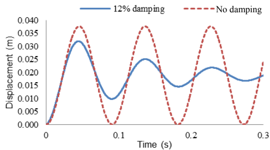
Fig. 12 Tip displacements of the 10-mm rubber plate under a suddenly applied constant 50 N force
