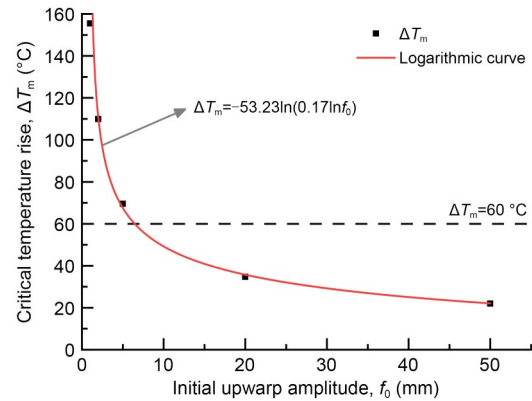
Fig. 13 Variation of \Delta T_m with f_0
