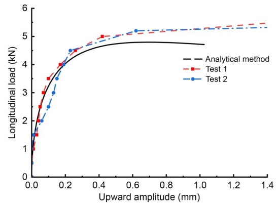
Fig. 9 Comparative verification of the upwarp buckling equilibrium path
