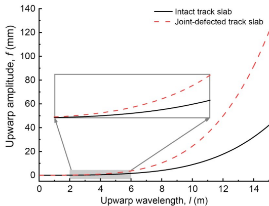
Fig. 11 Variation of upwarp amplitude f with upwarp wavelength l
