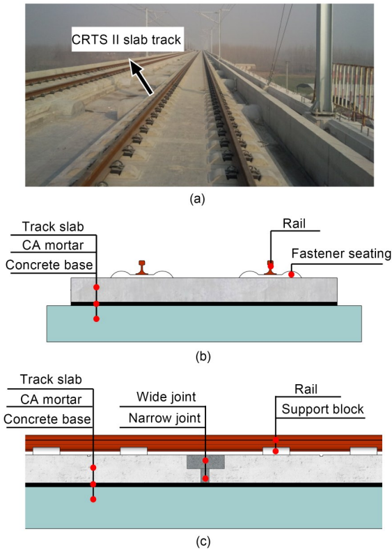
Fig. 1 Structure of the CRTS II slab track: (a) site photograph; (b) front view; (c) side view. References to color refer to the online version of this figure
