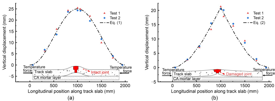
Fig. 5 Vertical displacement of the track slab model: (a) intact track slab model; (b) track slab model with a narrow joint defect
