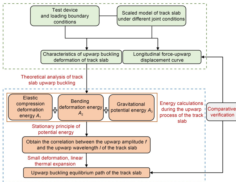
Fig. 6 Calculation workflow used in this study
