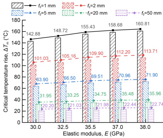
Fig. 18 Variation of \Delta T_m with elastic modulus
