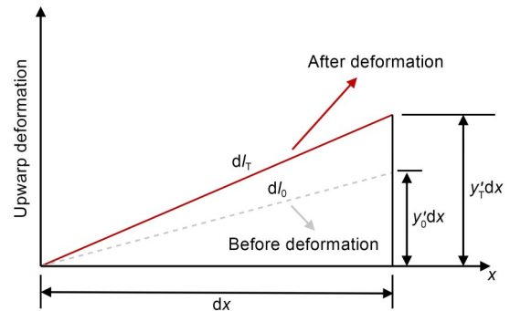
Fig. 8 Differences in the arc length of the track slabs before and after upwarp
