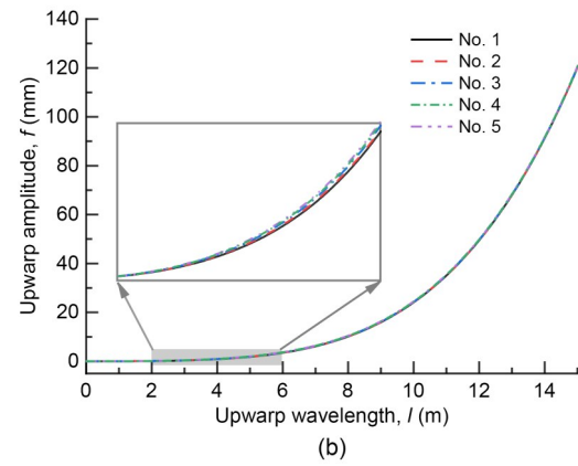
Fig. 15 Effect of the initial upward curve on the upward buckling of track slab: (a) upward buckling equilibrium path of the track slab; (b) variation of upward amplitude f with upward wavelength l
