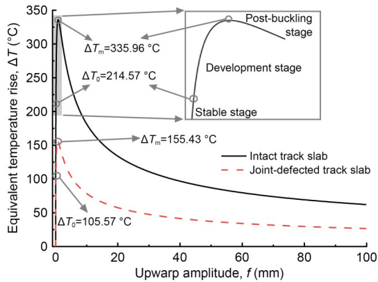
Fig. 10 Upwarp buckling equilibrium paths of the track slab without damage and with narrow joint defect
