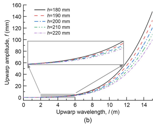
Fig. 21 Effect of track slab thickness on the upwarp buckling of the track slab: (a) upwarp buckling equilibrium path of the track slab; (b) variation of upwarp amplitude f with upwarp wavelength l
