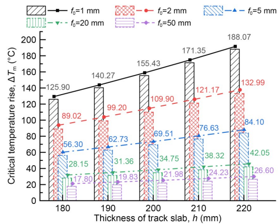
Fig. 22 Variation of \Delta T_m with track slab thickness
