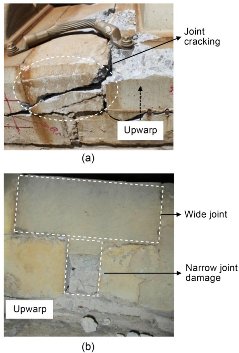
Fig. 2 Typical joint damage: (a) compression cracking; (b) defect and falling block
