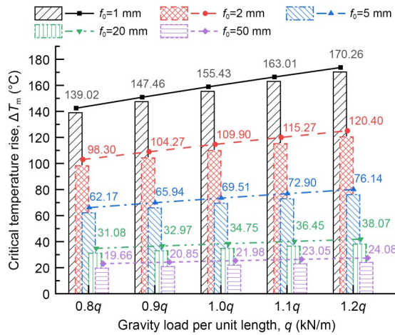
Fig. 20 Variation of \Delta T_m with gravity load
