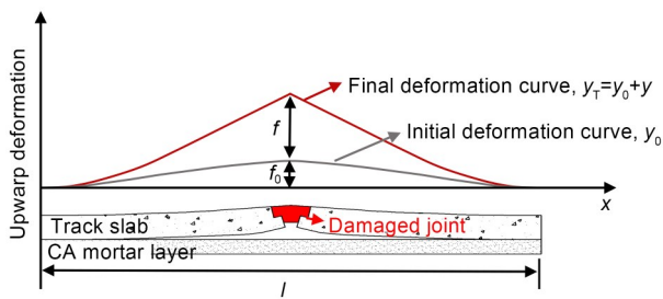
Fig. 7 Upward deformation of a track slab
