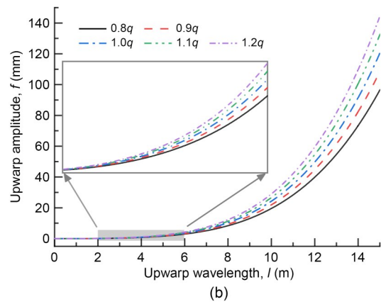
Fig. 19 Effect of the gravity load per unit length on the upwarp buckling of the track slab: (a) upwarp buckling equilibrium path of the track slab; (b) variation of upwarp amplitude f with upwarp wavelength l
