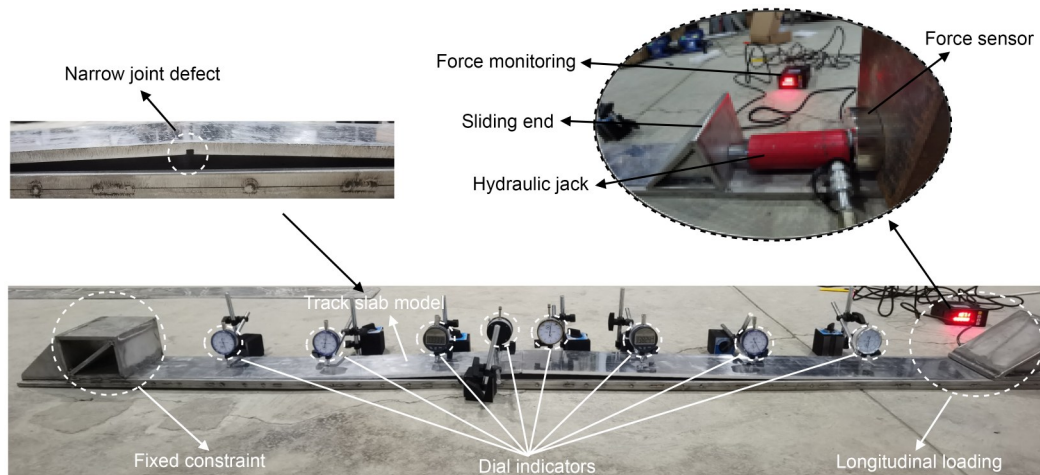
Fig. 4 Schematic diagram of the experimental test
