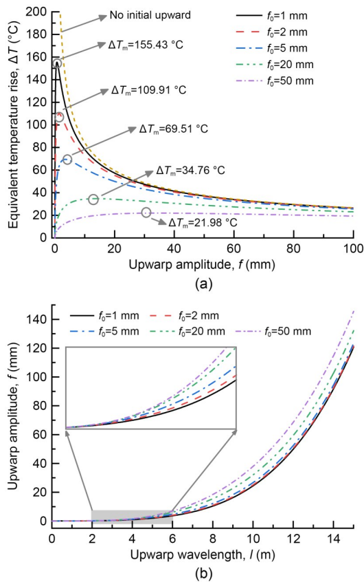
Fig. 12 Effect of f_0 on the upwarp buckling of track slab: (a) upwarp buckling equilibrium path of the track slab; (b) variation of upwarp amplitude f with upwarp wavelength l
