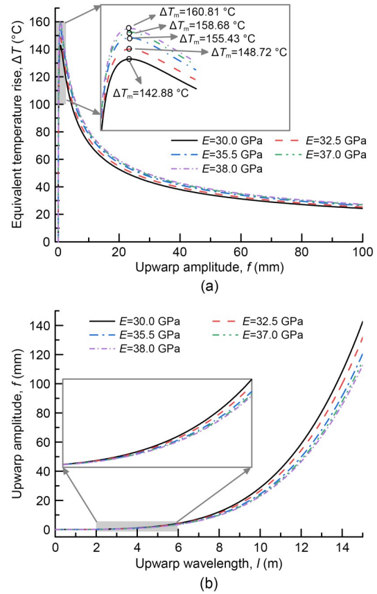
Fig. 17 Effect of elastic modulus on the upwarp buckling of the track slab: (a) upwarp buckling equilibrium path of the track slab; (b) variation of upwarp amplitude f with upwarp wavelength l
