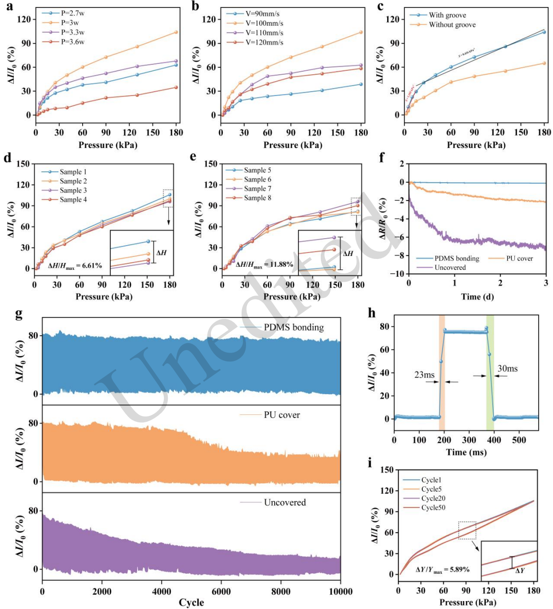
Fig. 3 Performance testing of the LIG pulse sensor. Relative current variation of sensors fabricated at different (a) laser powers and (b) scanning speeds under pressures ranging from 0 to 180 kPa. (c) Comparison of relative current changes at pressures ranging from 0 to 180 kPa for sensors with and without microgroove structures prepared at a laser power of 3 W and a scanning speed of 100 mm s -1 . Relative current changes at different pressures for four sensors from the same batch: (d) with MoS 2 modification and (e) without MoS 2 modification. (f) Initial resistance changes over 3 days for three sensor types: uncovered, directly covered with PU film, and chemically bonded with PDMS. (g) Relative current changes after over 10,000 loading/unloading cycles for three sensor types: uncovered, directly covered with PU film and chemically bonded with PDMS. (h) Response time and recovery time of the sensor at 100 kPa. (i) Changes in relative current and pressure during repeated loading and unloading cycles
