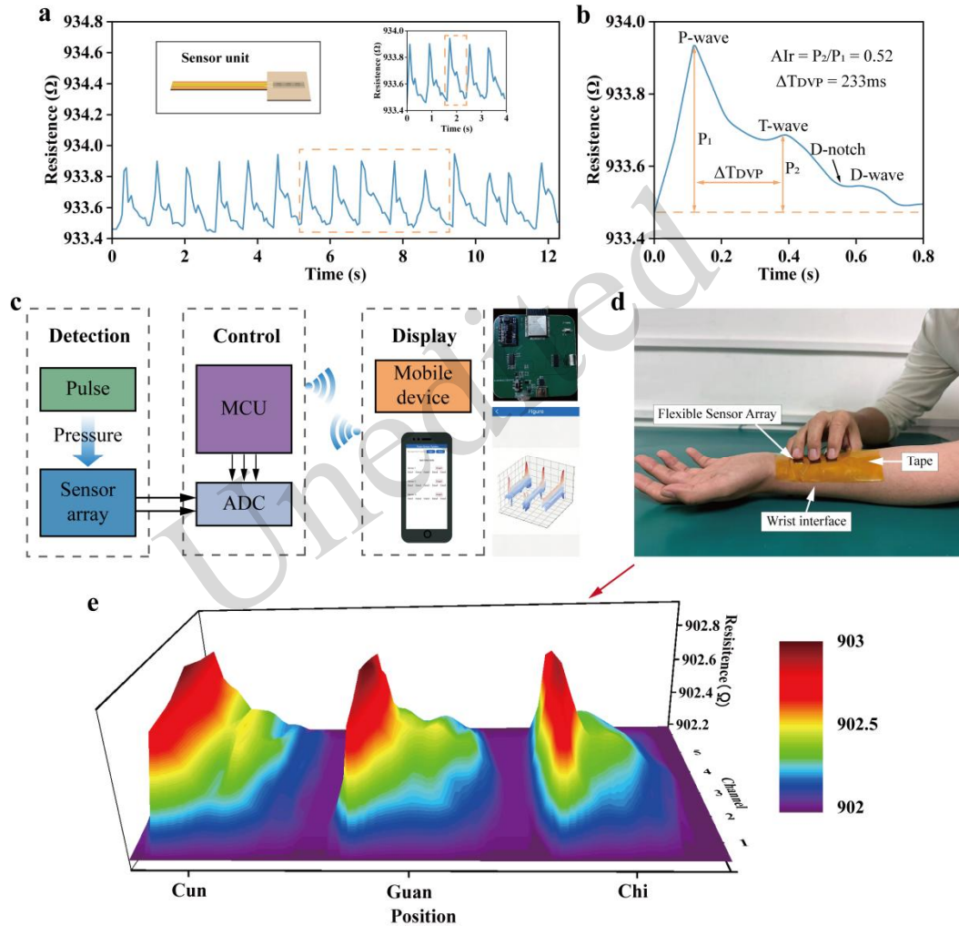
Fig. 4 Applications of the LIG Pulse Sensor. (a) Real-time arterial pressure waveform measured by the sensor at the wrist. The inset shows an image of the sensor placed on the wrist and a local schematic of five cycles. (b) Detailed image of the radial artery pulse wave during a single pulse cycle. (c) Schematic diagram of the signal acquisition system. (d) 3D pulse signal acquisition process. (e) 3D pulse signal image of a single pulse cycle
