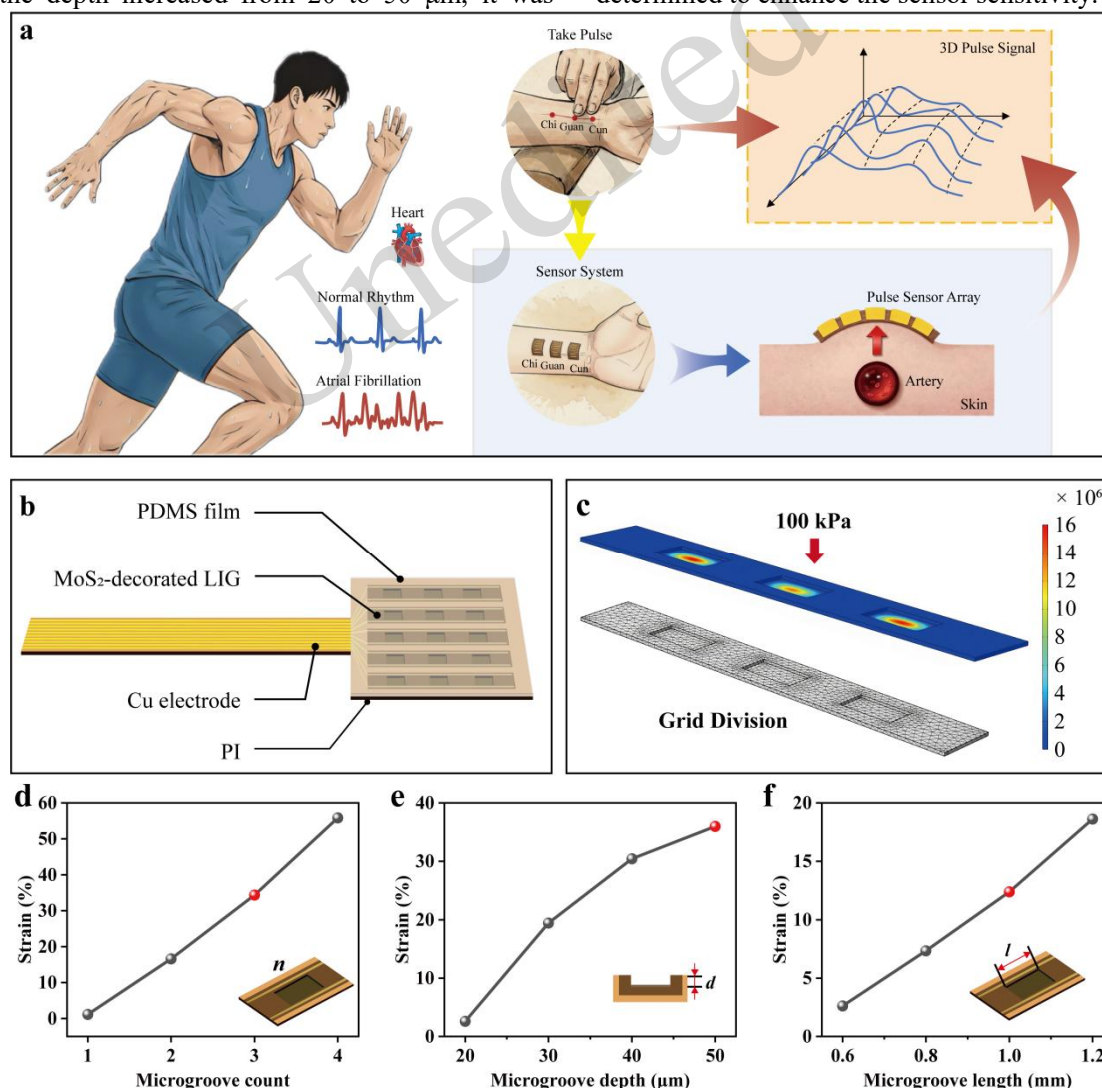
Fig. 1 Design of a 3D laser-induced graphene sensor. (a) Schematic of the sensor's operating mechanism. (b) Exploded view layout. (c) In situ stress distribution within the LIG at 100 kPa. Finite element analysis of the LIG yielded stress
