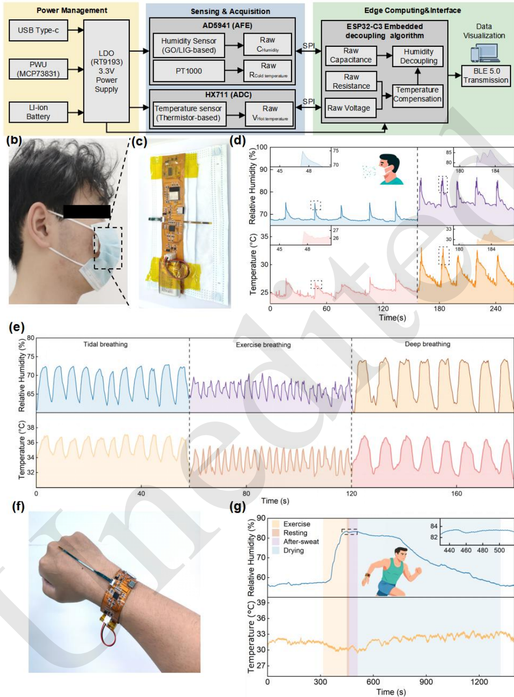
Fig. 5 Wearable physiological monitoring of respiration, coughing, and exercise. (a) Hardware architecture of the acquisition system based on an ESP32-C3 microcontroller. (b-c) Photographs of the sensor system attached to the inner surface of a commercial mask. (d) Response of the bimodal sensor to cough events. (e) Synchronized temperature-humidity waveforms during resting, exercise, and deep-breathing conditions. (f) Sensor system attached to the dorsal hand. (g) Dynamic evolution of skin temperature and humidity during exercise monitored by the sensor system
