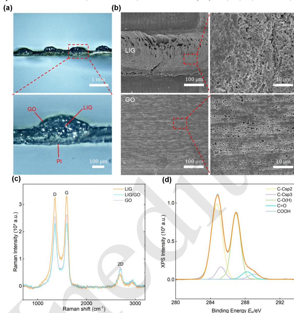
Fig. 2 Microstructural and compositional characterization of the sensing materials. (a) Cross-sectional optical micrograph showing intimate contact between LIG IDEs and GO film. (b) SEM images of the LIG IDE and GO film surfaces. (c) Raman spectra of LIG, GO, and LIG/GO composite materials. (d) High-resolution C 1s XPS spectrum of the GO film
