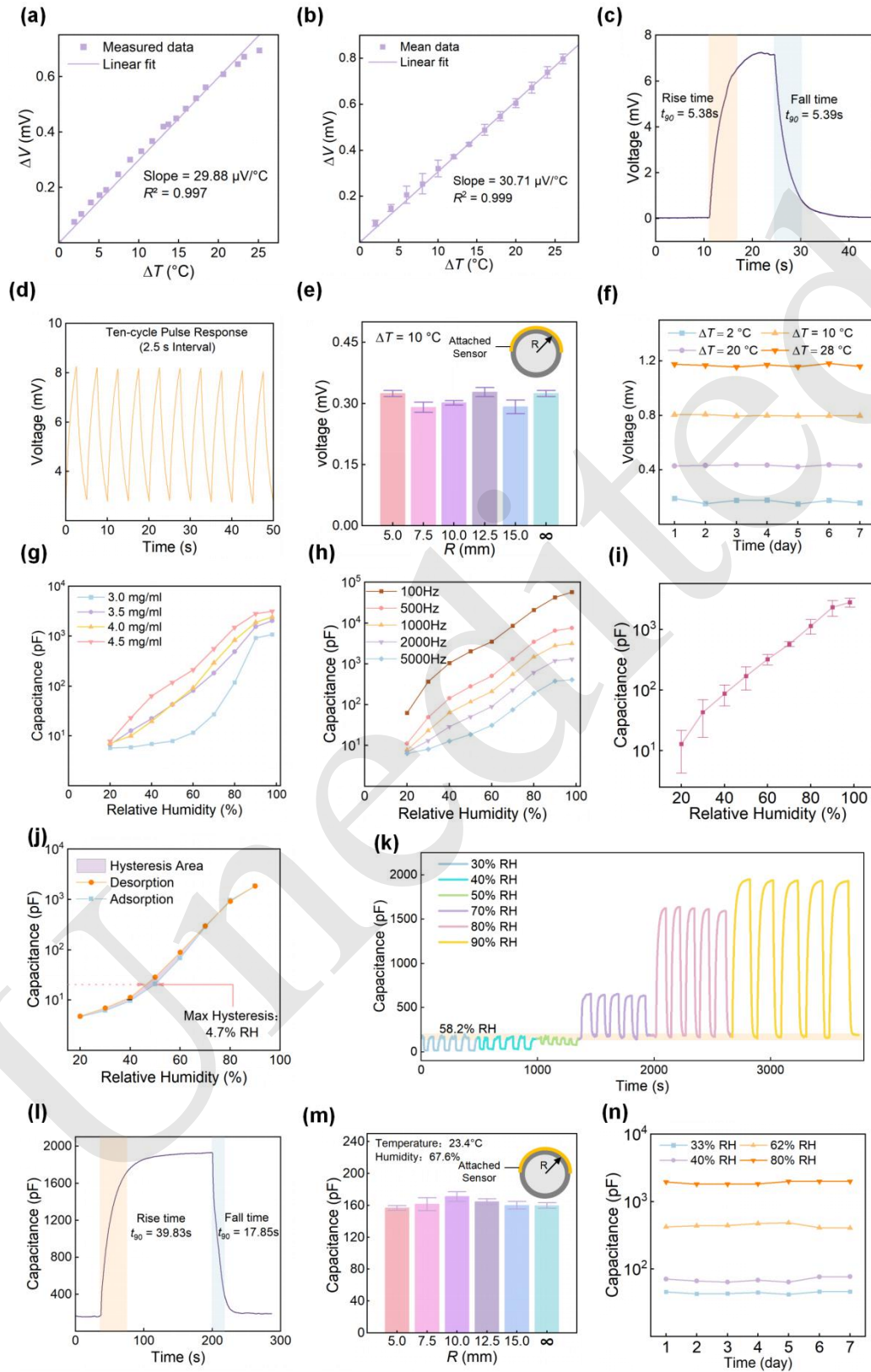
Fig. 3 Performance evaluation of the temperature and humidity sensing units. (a) Calibration curve and linear fit of the thermoelectric voltage ( \Delta V ) versus temperature difference ( \Delta T ) for a representative copper-constantan thermocouple. (b) Sample-to-sample reproducibility of the temperature sensor, showing the mean thermoelectric response and standard
