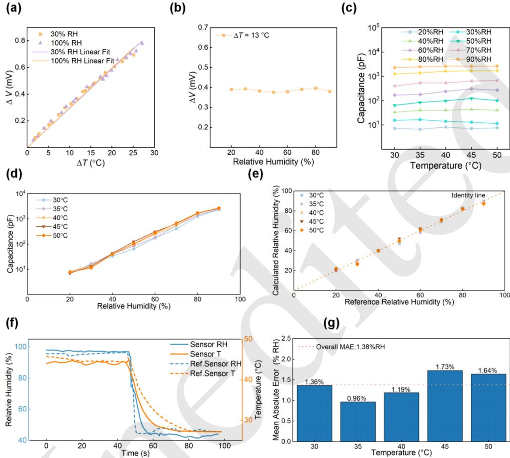
Fig. 4 Crosstalk evaluation and decoupling via a second-order polynomial model. (a) Calibration of the temperature sensor under environments with distinct relative humidity levels of 30% and 100%. (b) Response of the temperature sensor to a constant hot-to-cold junction temperature difference of 13 °C as the relative humidity increases from 20% to 90%. (c) Responses of the humidity sensor at specific relative humidity levels as the temperature increases from 30 °C to 50 °C. (d) Raw experimental dataset used to establish the second-order polynomial regression model. (e) Comparison between the compensated humidity measurement results and the ideal reference line. (f) Dynamic decoupling performance under a simultaneous wide-range temperature-humidity transition from 44.6 °C/98% RH to 27.2 °C/43% RH, compared with a commercial reference sensor. (g) Mean absolute errors of humidity measurements at different temperatures after algorithmic compensation
