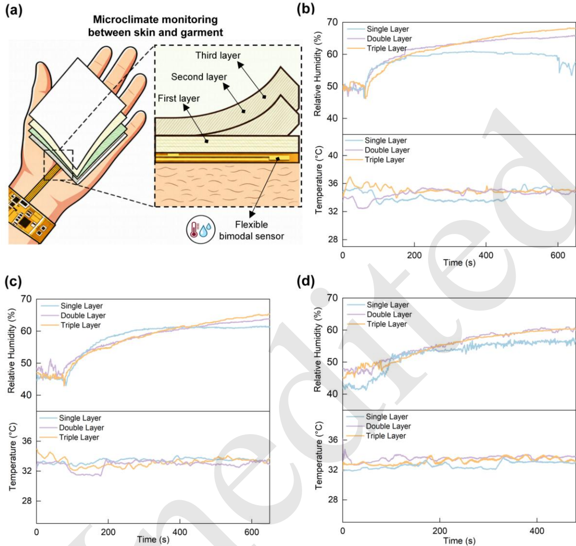
Fig. 6 (a) Schematic illustration of the skin-garment microclimate test configuration with varying fabric layers (single, double, and triple layers). (b-d) Simultaneous real-time measurements of relative humidity and temperature at the skin-garment interface for (b) 100% polyester, (c) a 50/50 polyester-cotton blend, and (d) 100% cotton fabrics
